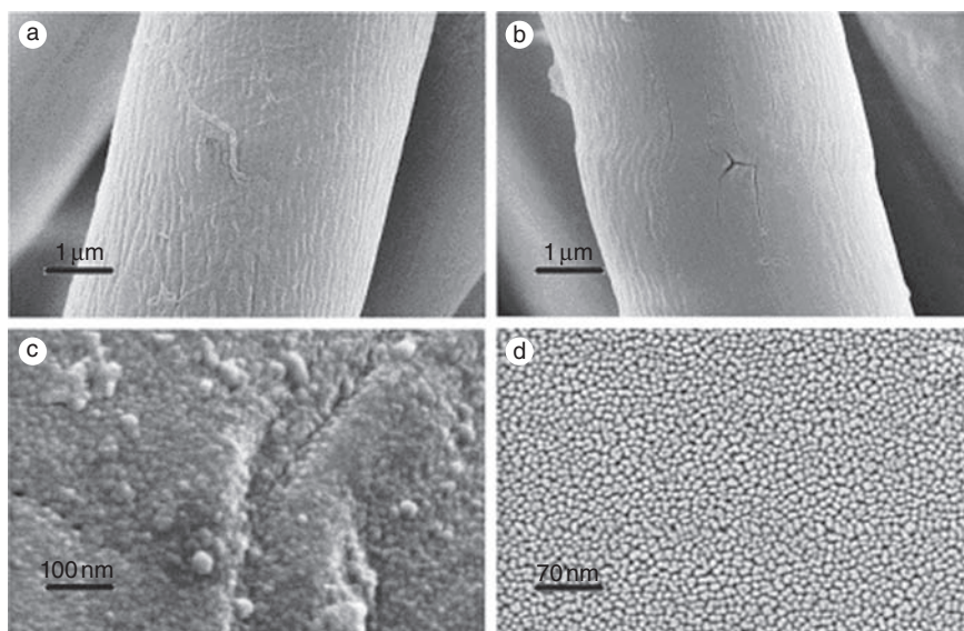
13.6 SEM images of (a) uncoated cotton fiber, (b) titania coated cotton fiber showing the morphological change in the surface structure, (c) higher magnification image of titania coated cotton fiber showing the shape and size of the titania particles, and (d) higher magnification image of a titania film coated on glass [7].
