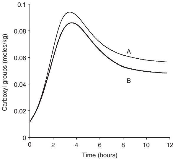
4.12 Calculated carboxylic acid end group [\text{COOH}] concentration in a typical VK tube: (A) considering the effect of increasing hydrostatic pressure inside the reactor; and (B) assuming constant atmospheric pressure throughout the reactor.
