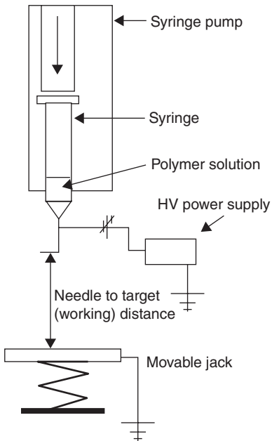
13.19 Schematic diagram of electrospinning set-up [153].
