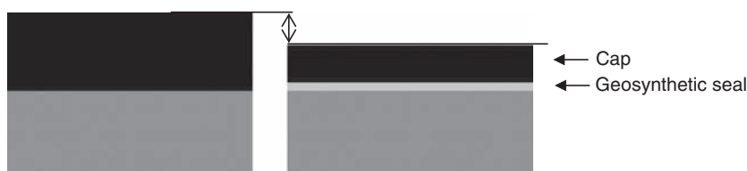
18.16 Pavement reduced thickness by reducing the asphalt cap thickness (adapted [43]).
