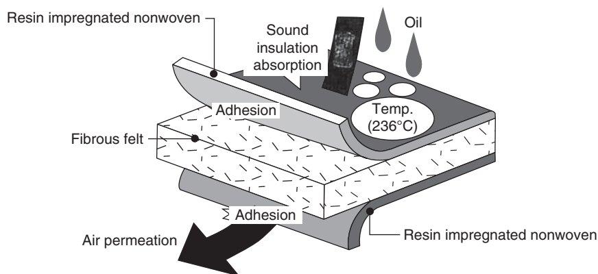
17.10 An example of an engine silencer. 16
