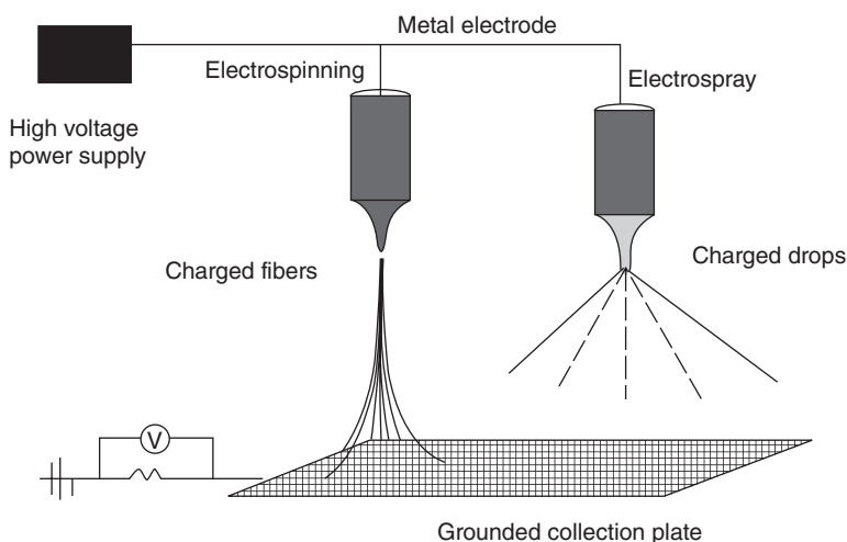
13.21 Electrospaying and electrospinning set-up [147].
