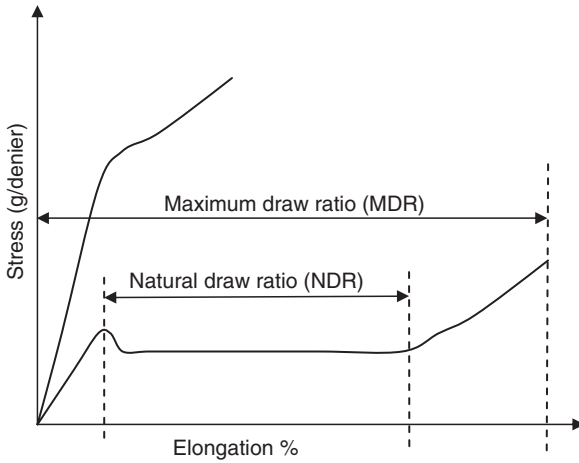
4.20 Stress–strain curves for as-spun and spun-drawn fibre.
