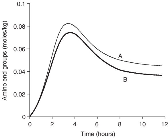
4.11 Calculated amino end group [\text{NH}_2] concentration in a typical VK tube: (A) considering the effect of increasing hydrostatic pressure inside the reactor; and (B) assuming constant atmospheric pressure throughout the reactor.
