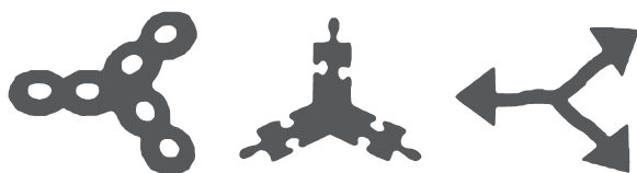
7.5 Cross sections with high shape factor.
