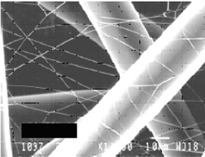
13.25 Ultraweb – nanofiber filter media from Donaldson [170].
