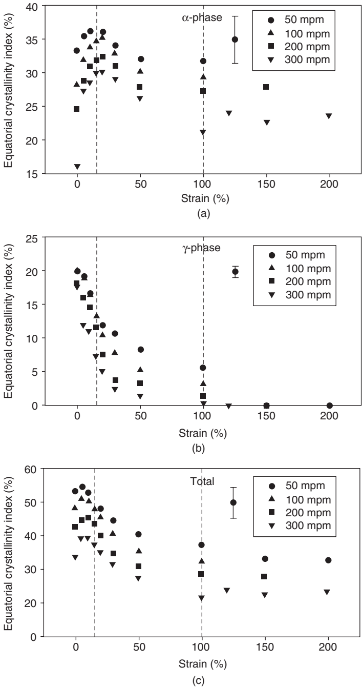
4.22 The equatorial crystallinity index (ECI) as a function of take-up speed and strain percentage of the: (a) \alpha -phase; (b) \gamma -phase; and (c) total ( \alpha + \gamma ); MPM = metres per minute.
