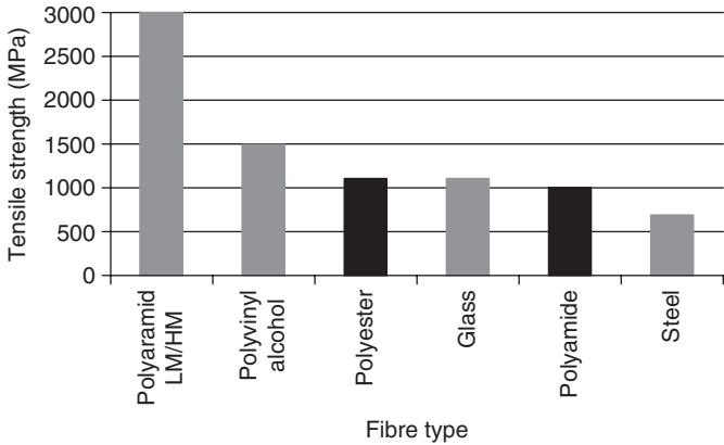
18.5 Tensile strength of fibres used to reinforce concrete (LM: low modulus; HM: high modulus).
