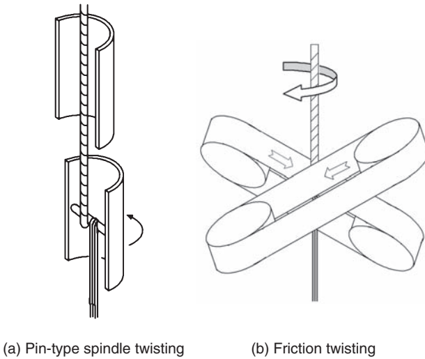
3.13 The mechanism of false-twist types.
