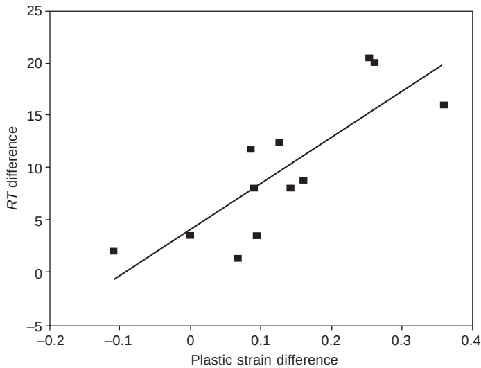
4.15 Relationship between DRT and D\epsilon .
