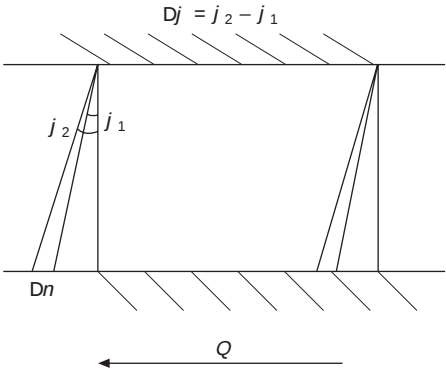
6.15 Determination of Dn .
