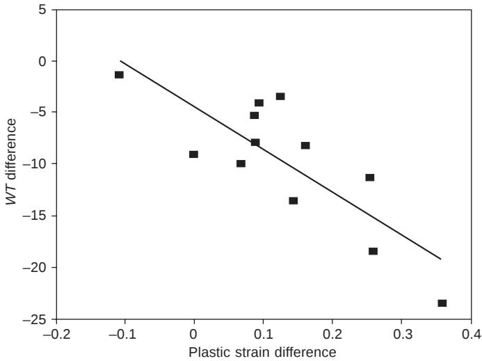
4.14 Relationship between DWT and De .
