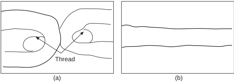
8.16 Cross-section of a fabric strip (¥ 200) with (a) a vertical plain seam and (b) no seam.
