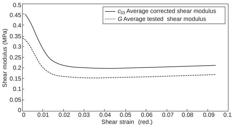
6.19 Comparison of simple and modified shear moduli.
