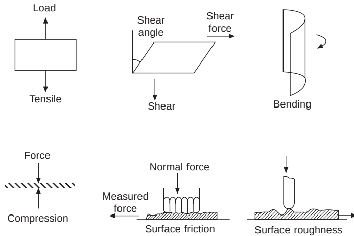
2.1 Measuring principles of the KES system.
