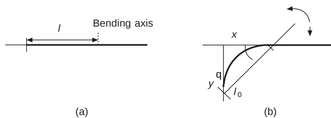
8.6 Measurement of bending angle q and chord l_0 ; (a) before deflection; (b) during deflection.
