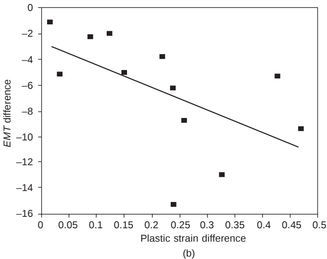
4.13 Relationship between DEMT and De for (a) circular cross-section and (b) elliptic cross-section.
