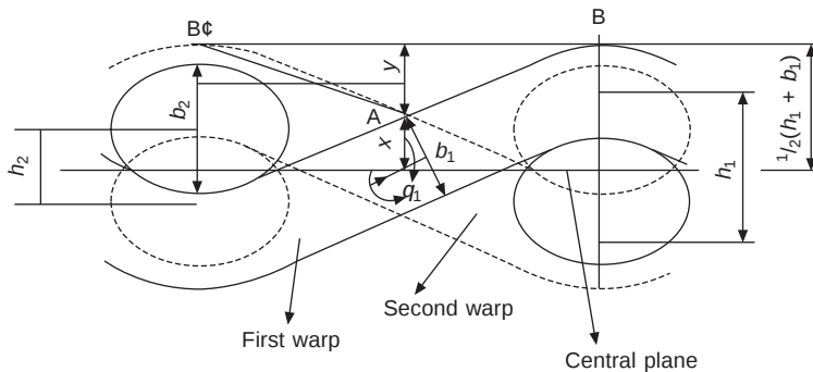
3.14 Geometrical roughness of woven fabrics.
