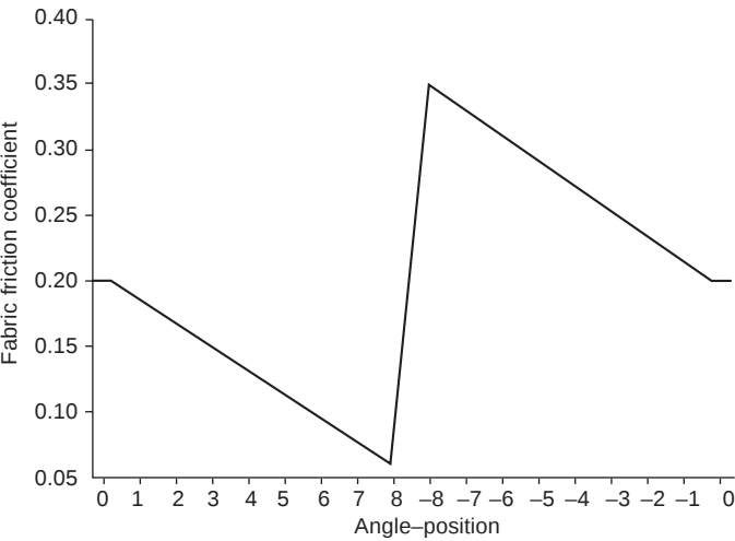
3.19 Predicted friction variation when m_f = 0.2 .
