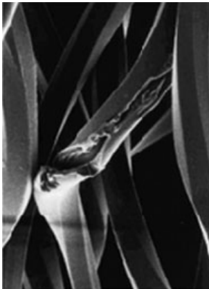
5.2 Filament tear due to cool track edge contact.
