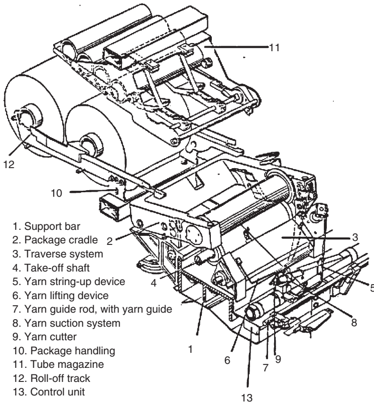
5.27 Example of automatic doffing module (two-pack storage) (Barmag AFK) (Illustration © Oerlikon-Barmag).
