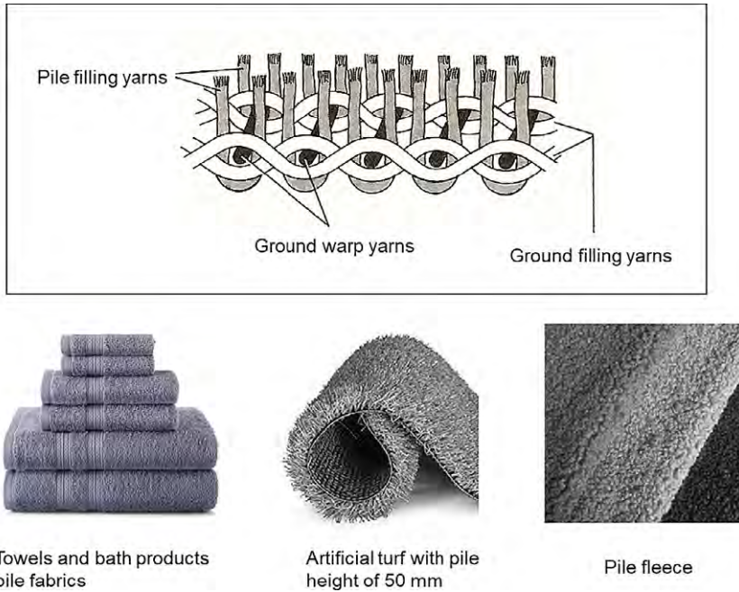
Fig. 10.3 Pile fabrics and product examples.
