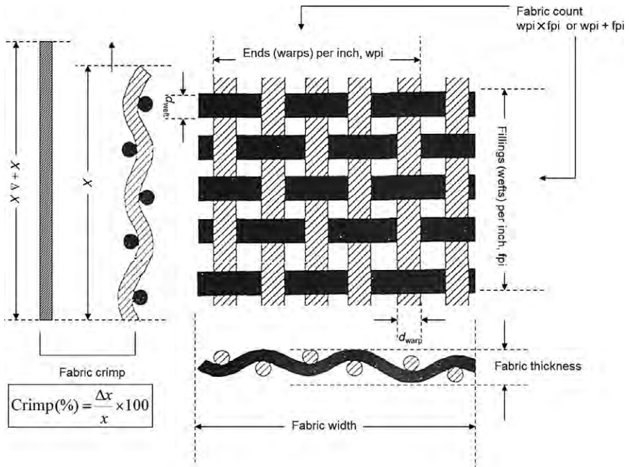
Fig. 10.6 Woven fabric basic specifications [3–7].
