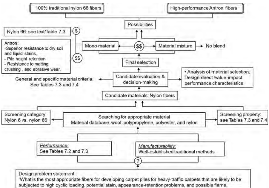
Fig. 7.8 Material selection steps for carpet pile fibers.
