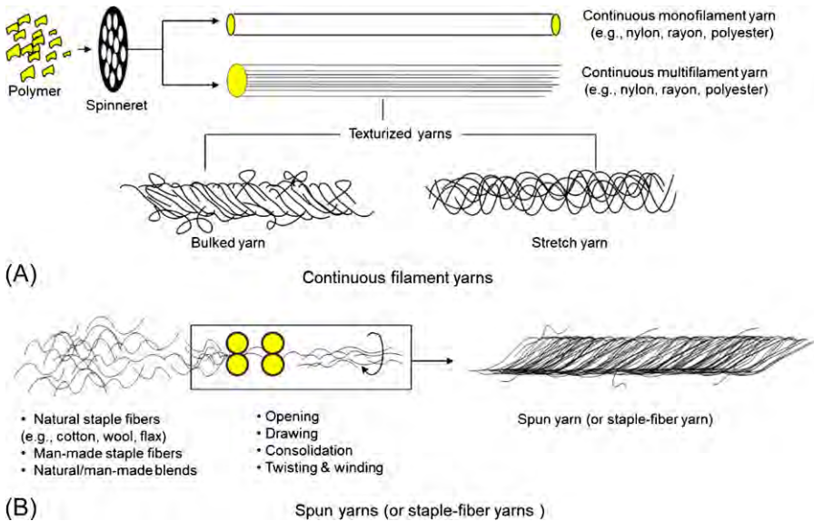
Fig. 9.1 Continuous-filament yarns and spun (staple-fiber) yarns.
