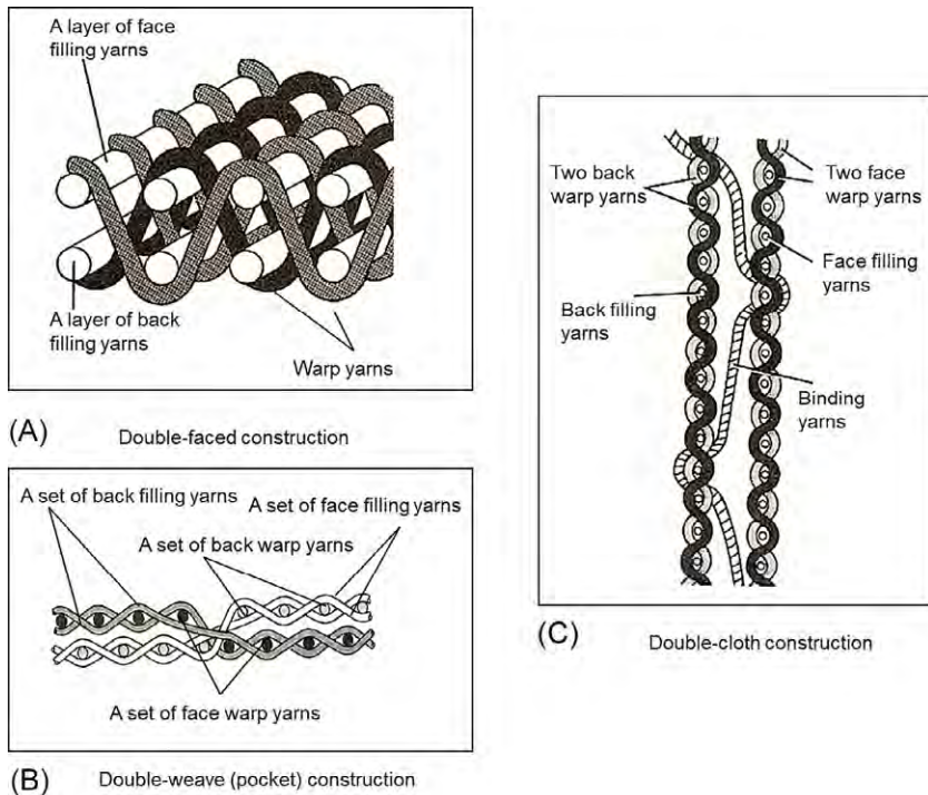
Fig. 10.4 Constructions of double woven fabrics [4–6].
