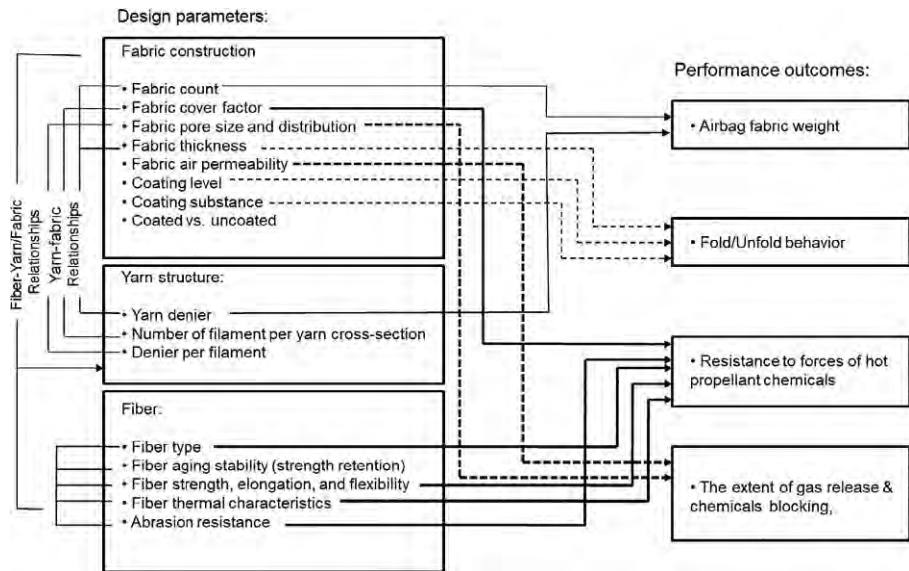
Fig. 15.6 Design parameters and related performance outcomes of airbag fabric.
