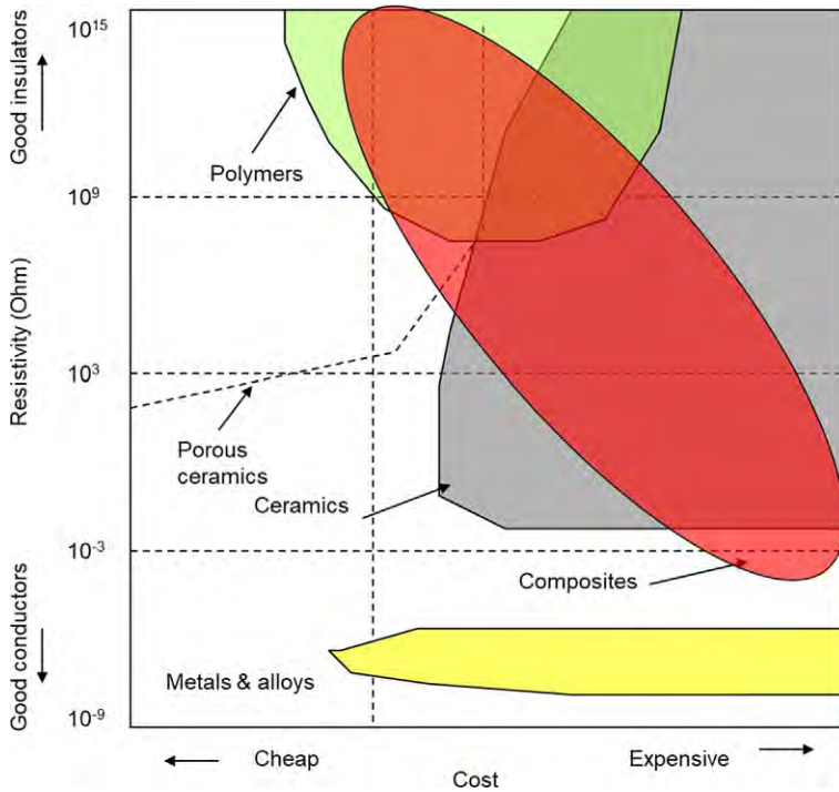
Fig. 7.6 Electrical resistivity versus estimated cost of different materials. Modified from Cambridge Material Charts, Department of Mechanics, Materials, Design, United Kingdom, 2002. http://www-materials.eng.cam.ac.uk/mpsite/interactive_charts .
