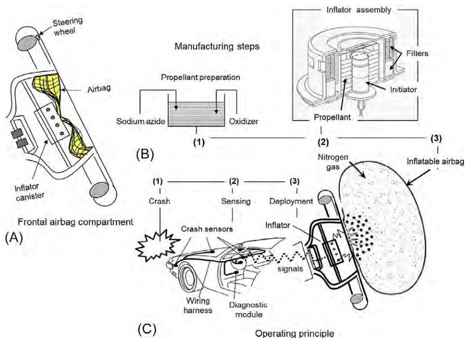
Fig. 15.3 Basic components of airbag (schematics assembled from different auto-maker sources).
