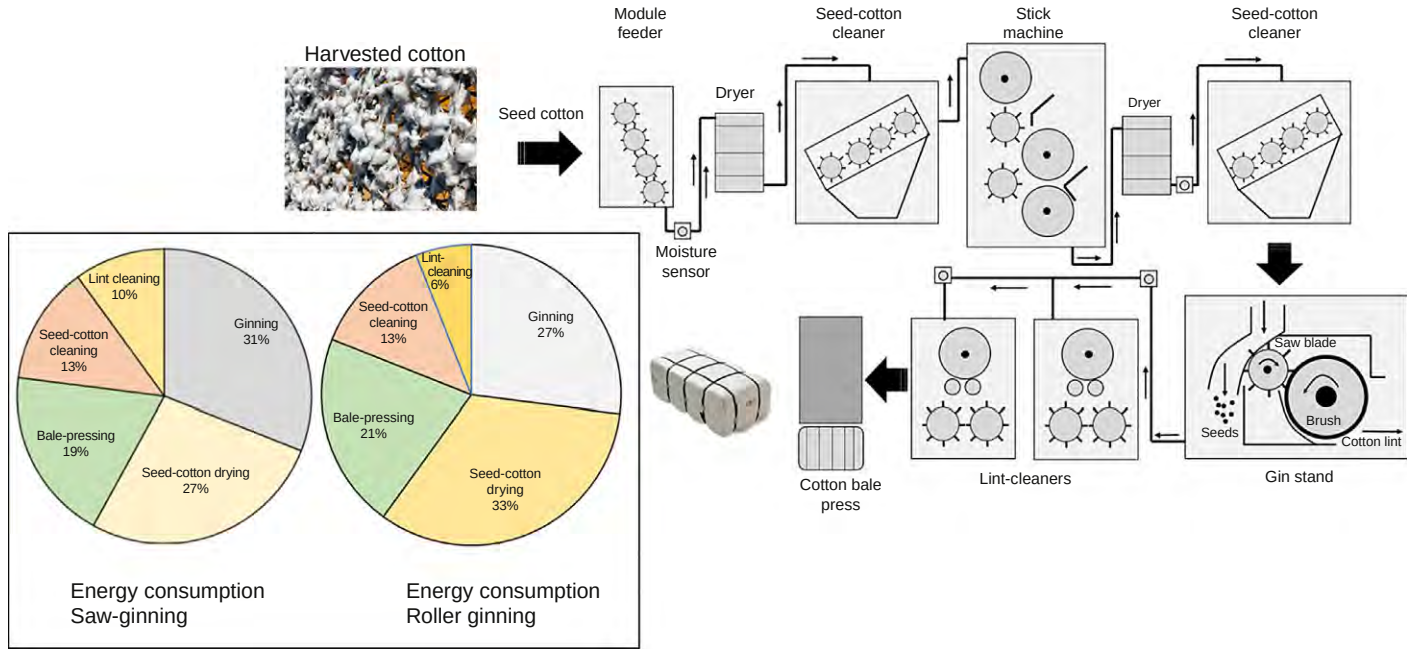
Fig. 6.4 Flow of seed cotton through the ginning process energy distribution derived from Refs [42–44].
