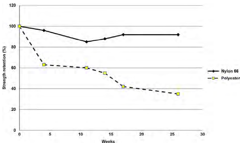
Fig. 15.5 Comparison between uncoated nylon 66 and polyester fabric tensile strength retention after aging test.
