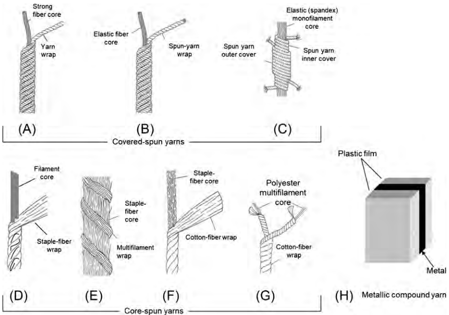
Fig. 9.3 Examples of compound (or composite) yarns [1,4,7] .
