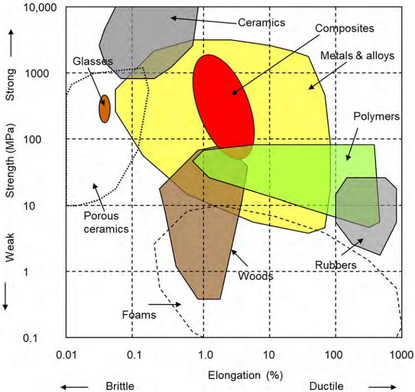
Fig. 7.4 Yield strength-elongation of major material categories.
