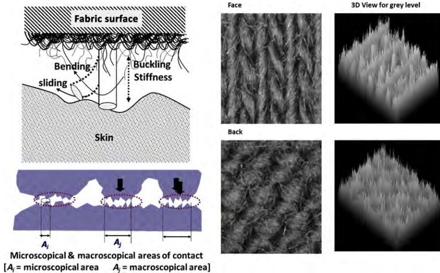
Fig. 5.3 Examples of structural- and design-related parameters revealed in the area-ratio model [67–70].
