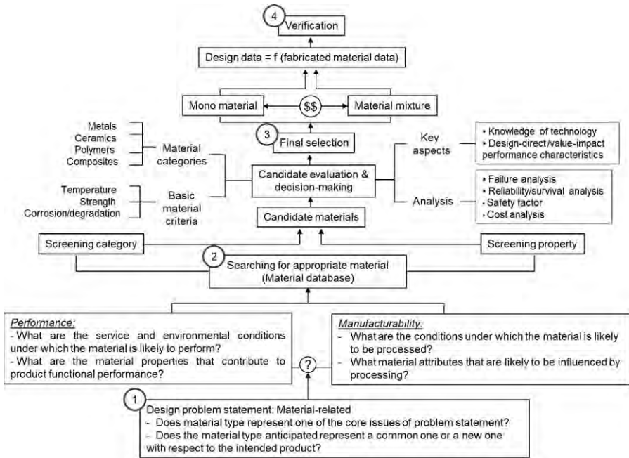
Fig. 7.1 Basic material selection steps.
