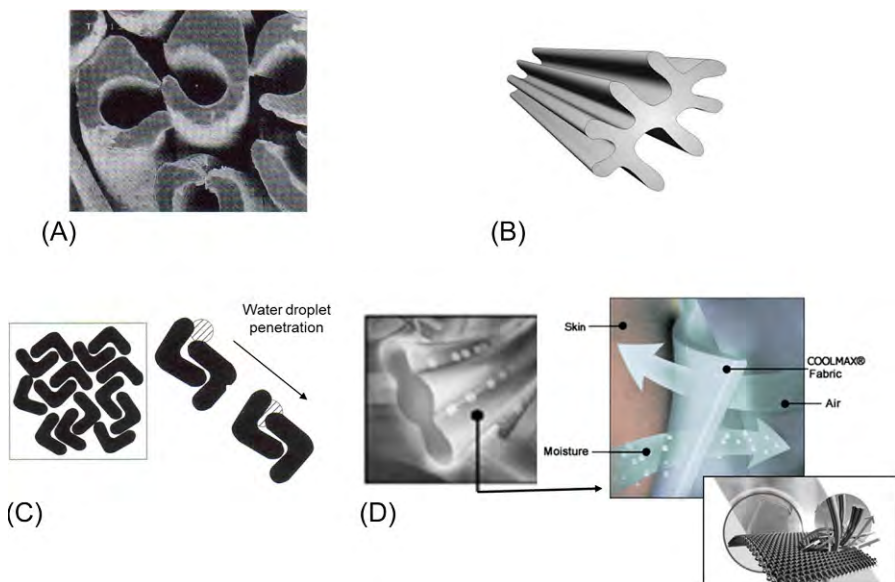
Fig. 13.6 Specialty cross-sectional shapes [21–25]. (A) C-Slit. “Killat N”-Kanebo Ltd.; (B) 4DG Eastman Chemical; (C) L-Shaped Nylon Cross-Section “Ciebet”-Asahi Chemical Industry Co., Ltd.; (D) Four-channel fiber (COOLMAX).
