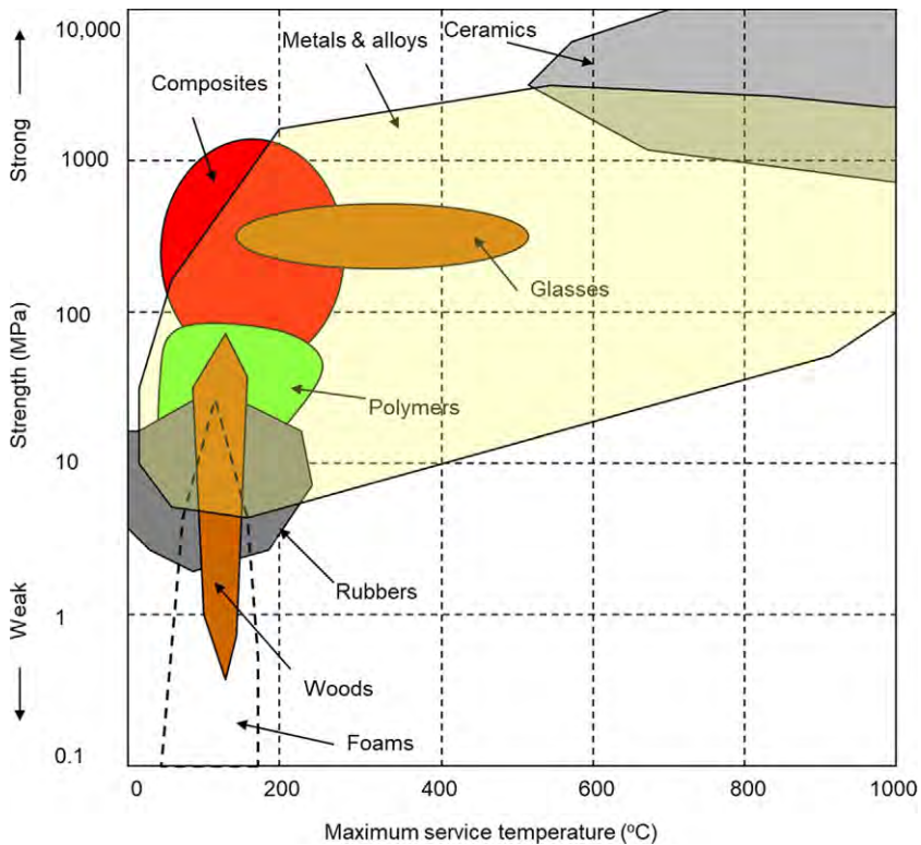
Fig. 7.5 Yield strength-temperature of major material categories.
