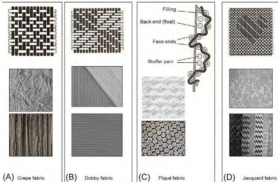
Fig. 10.2 Special woven constructions.
