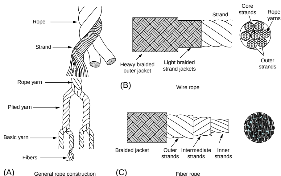
Fig. 9.5 Rope constructions [15–17].
