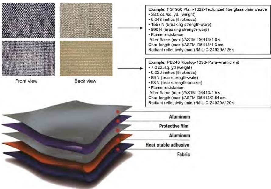
Fig. 16.11 Example of protective fibrous products used for extreme climates Gentex's proprietary Dual Mirror/Flexir aluminized fabric ( http://www.Gentexcorp.com ).
