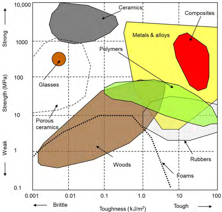
Fig. 7.3 Yield strength-toughness of major material categories.
