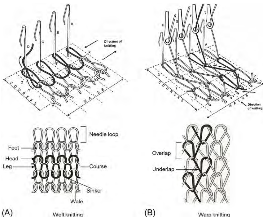
Fig. 10.7 Basic knit structures [6,10,11].
