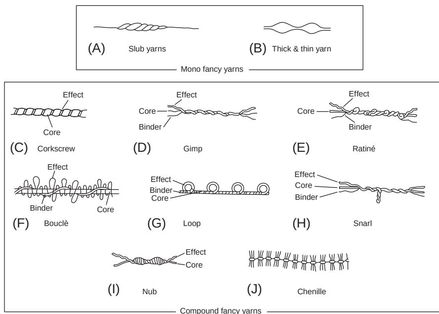
Fig. 9.6 Examples of fancy yarns [4,7,18].
