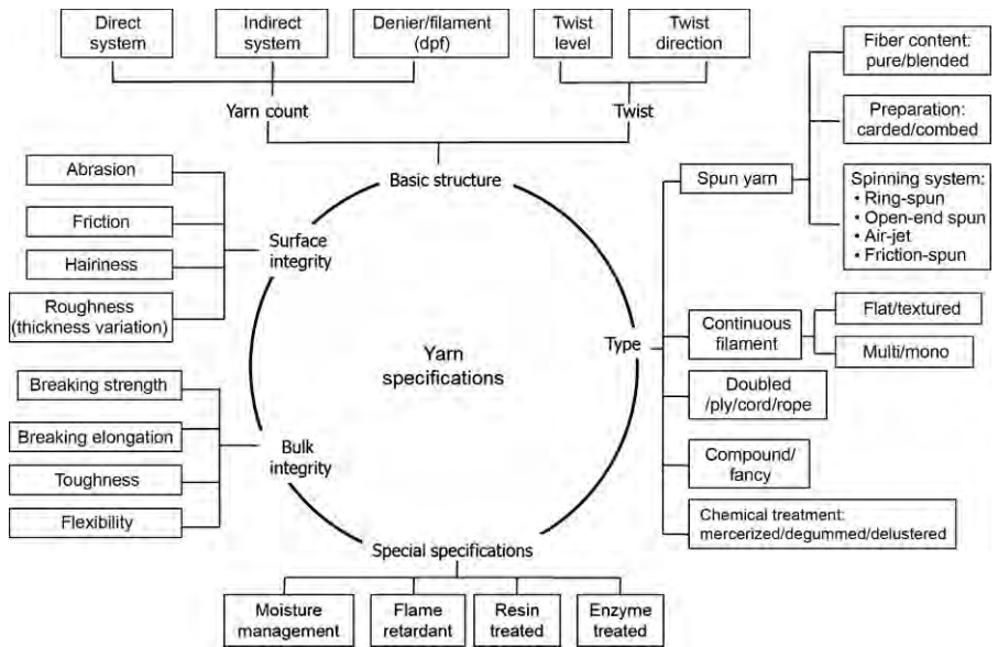
Fig. 9.2 Common yarn specifications.
