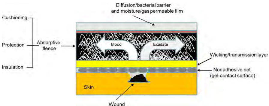
Fig. 16.2 Basic structure of wound dressing laminate.
