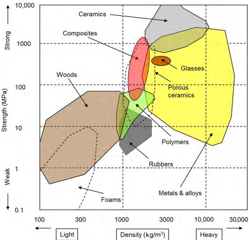
Fig. 7.2 Yield strength-density of major material categories.
