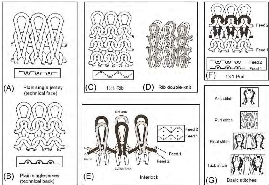
Fig. 10.8 Weft-knit structures [12–15].
