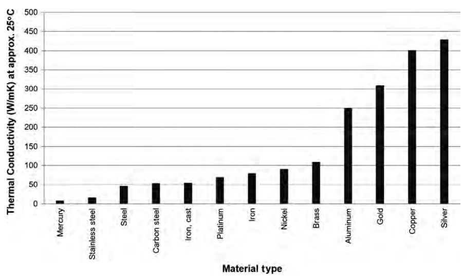
Fig. 8.11 Typical values of thermal conductivity of highly conductive materials. Based on data from R.B. Seymour, Engineering Polymer Sourcebook , McGraw-Hill, NY, 1990; W.F. Smith, Materials Science and Engineering , AccessScience@McGraw-Hill, 2001, doi:10.1036/1097-8542.409550. http://www.accessscience.com , last modified: May 4; C.E. Carraher, Jr., Polymer , AccessScience@McGraw-Hill, 2004, doi:10.1036/1097-8542.535100. http://www.accessscience.com , last modified: March 12.
