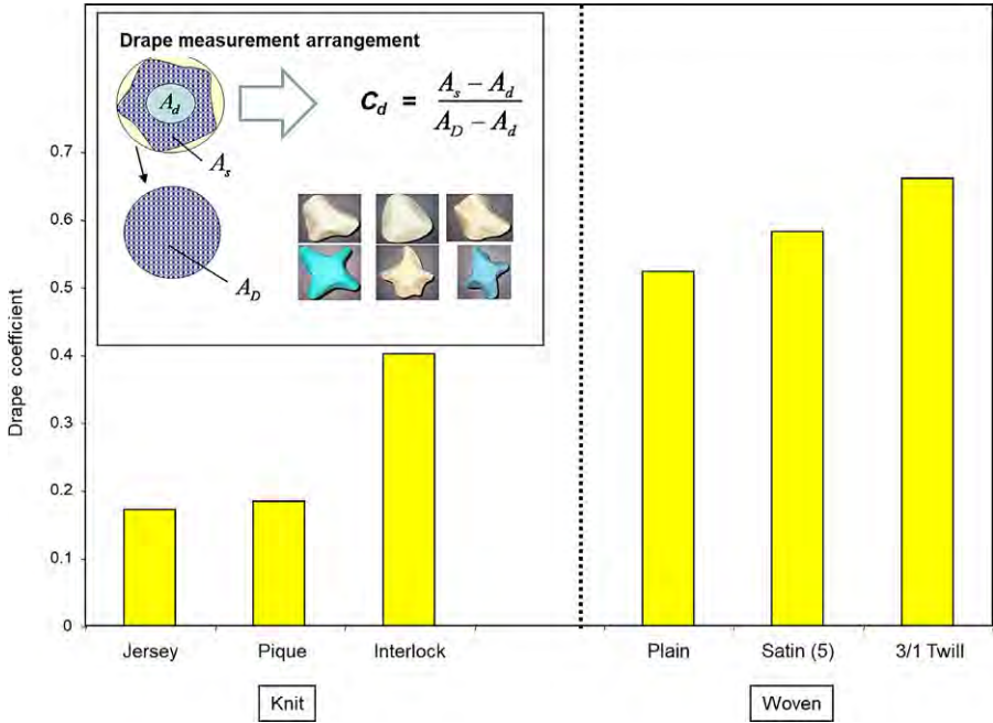
Fig. 12.3 Drape coefficient of different 100% cotton fabrics [33].
