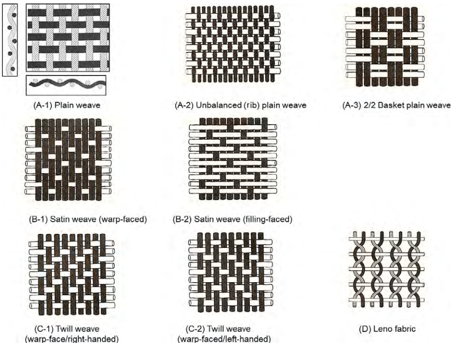
Fig. 10.1 Basic woven structures [1–6].
