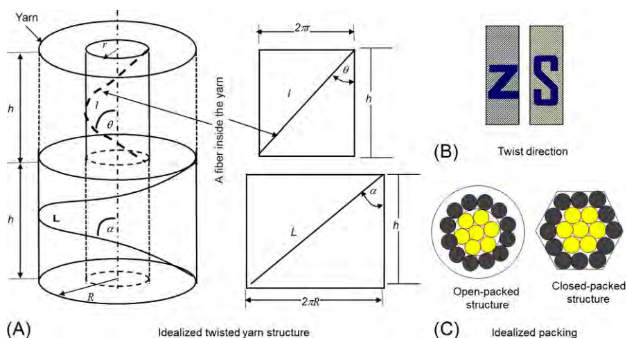
Fig. 9.7 Twist in idealized yarn structure.
