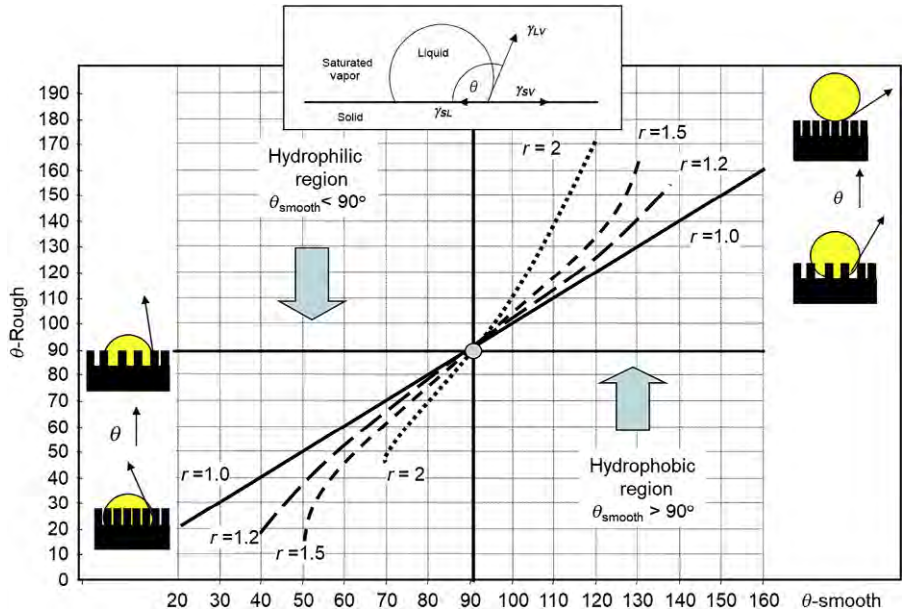
Fig. 11.1 Demonstration of Young and Wenzel models [21–25]. In the hydrophilic material (left), as r increases from 1 to 2, \theta decreases. In the hydrophobic material (right), as r increases from 1 to 2, \theta increases.
