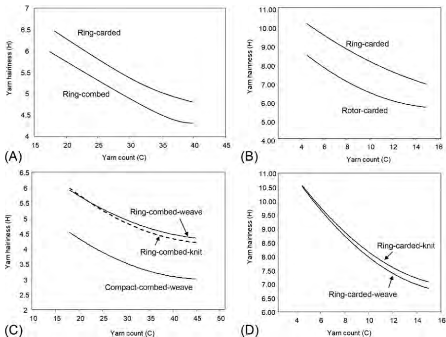
Fig. 9.9 Uster yarn hairiness at different preparations and different spinning methods.
