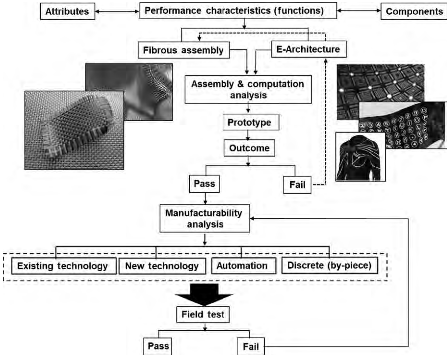
Fig. 14.1 General design scheme of E-textiles.
