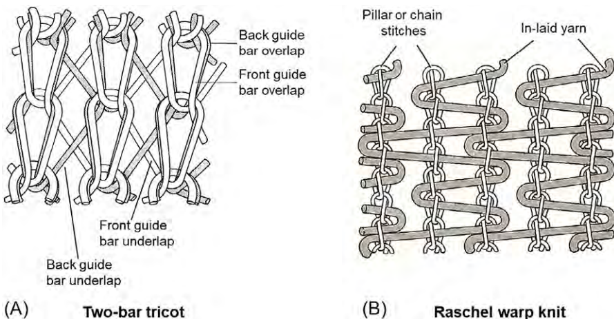
Fig. 10.9 Warp-knit structures [12–15].
