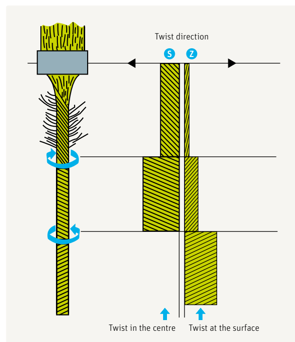
Fig. 29 – The distribution of twist in the running fiber strand
