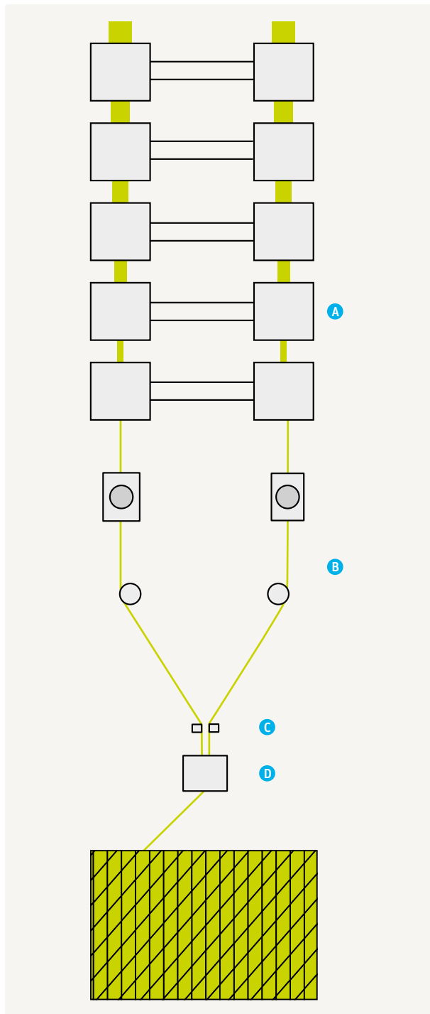
Fig. 32 – The PLYfL spinning system
