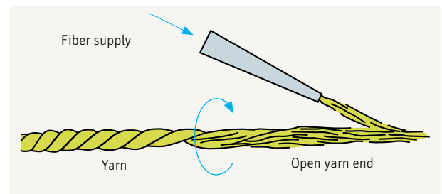
Fig. 1 – Formation of an open-end spun yarn
