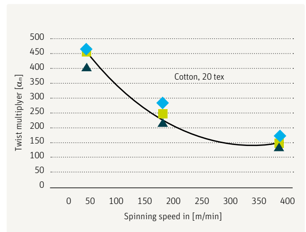
Fig. 39 – Yarn twist as a function of spinning speed (Rieter)
