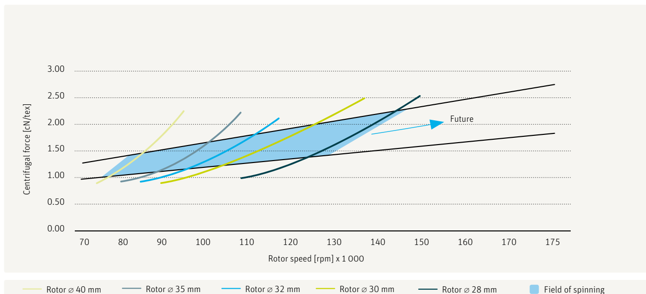
Fig. 18 – Centrifugal force as a function of rotor diameter and rotor speed
