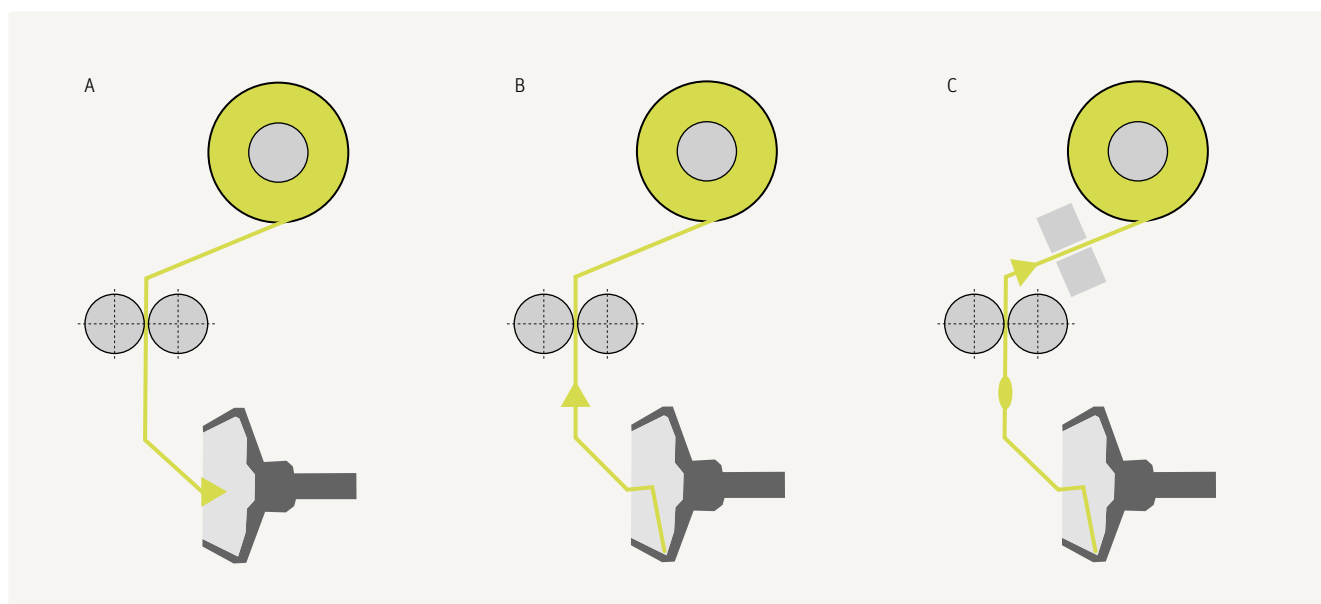
Fig. 55 – Automatic piecing after an end down or quality stop
