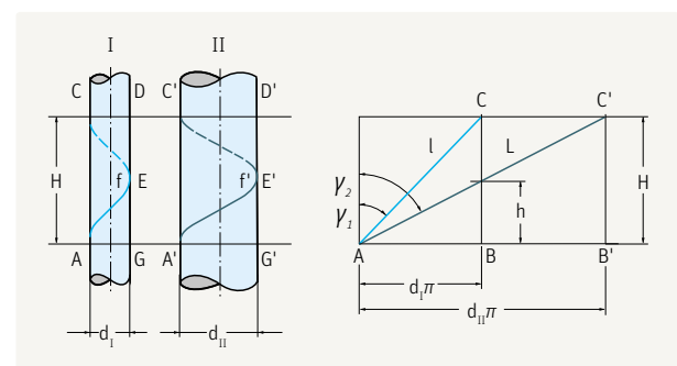
Fig. 90 – Angle of inclination of fibers in two yarns of differing thickness
