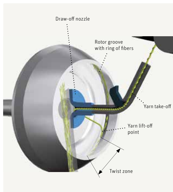
Fig. 17 – Yarn formation and twist insertion in the rotor groove
