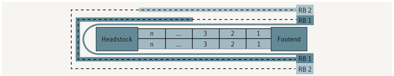
Fig. 49 – Travel strategy with one operating robot on each side of the machine; each robot can also serve the other side
