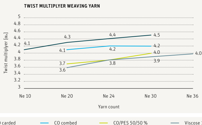
Fig. 91 – Twist multipliers customary in mill practice for rotor-spun weaving yarns
