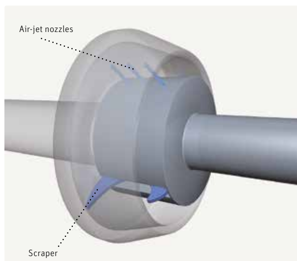
Fig. 20 – Rotor cleaning module with Air-jet nozzles and scrapers
