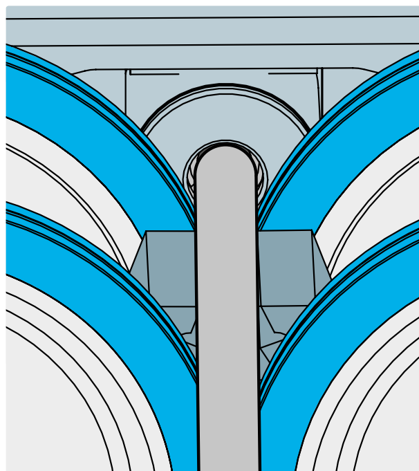
Fig. 22 – Support-disc bearing (Twindisc bearing) with rotor fitted
