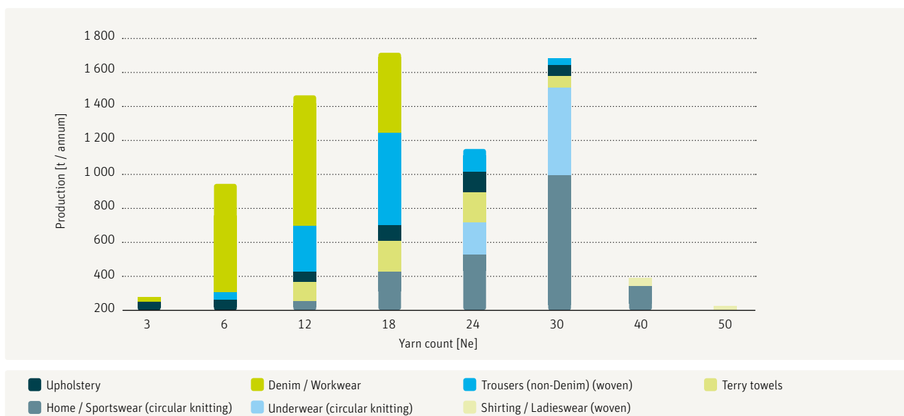
Fig. 5 – Annual output (tonnes worldwide) of end products from rotor-spun yarns, by yarn count
