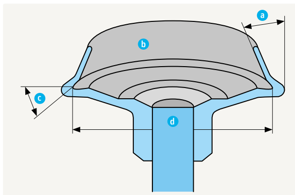
Fig. 74 – Important rotor parameters: rotor wall (a), surface of the rotor wall (b), rotor groove (c) and groove diameter (d)
