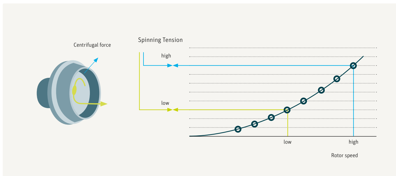
Fig. 57 – Influence of piecing speed on spinning tension and thus on piecing tenacity
