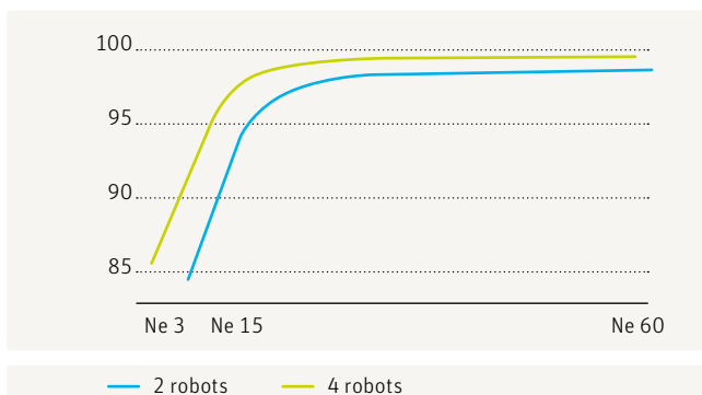
Fig. 51 – Machine efficiency with 2 and 4 robots
