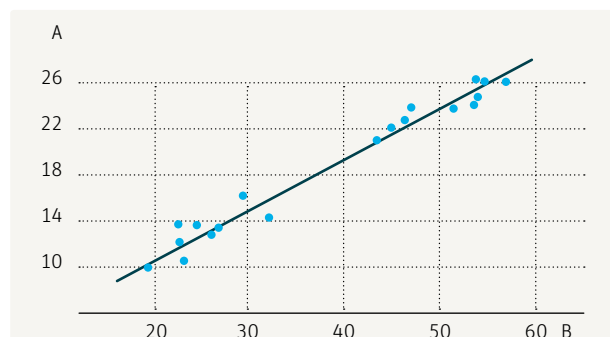
Fig. 70 – Relationship between fiber tenacity (B) and yarn tenacity (A) in cN/tex
