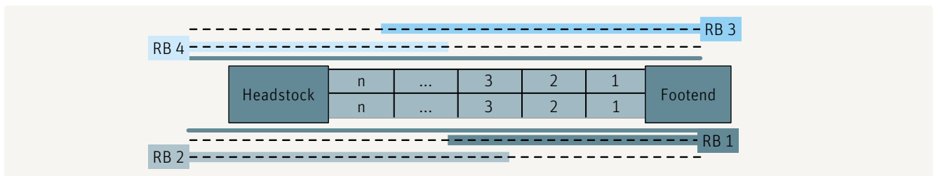
Fig. 52 – Travel strategy with 2 robots on each side of the machine
