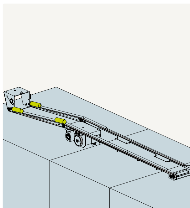
Fig. 40 – Supplying empty tubes via conveyor belts
