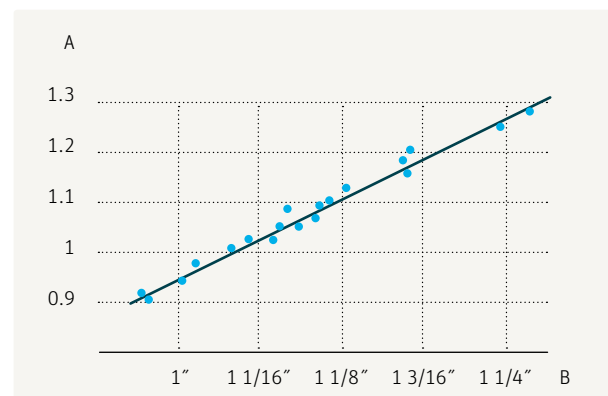
Fig. 69 – Relationship between staple length in inches (B) and yarn tenacity (A)
