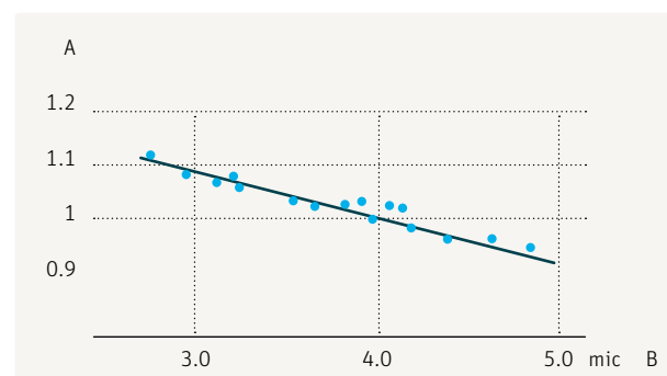
Fig. 68 – Relationship between fiber count (B) and yarn tenacity (A)
