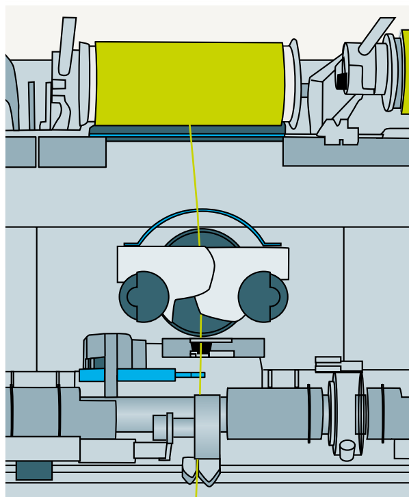
Fig. 31 – Winding head with package
