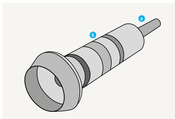
Fig. 21 – Direct rotor bearing, with rotor shaft (a) encased in ball bearing housing (b)
