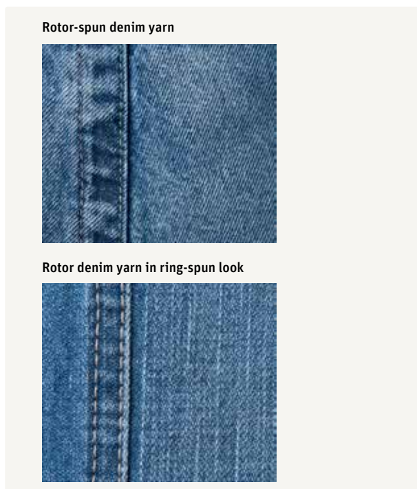
Fig. 87 – Fabric woven from rotor-spun denim yarn
