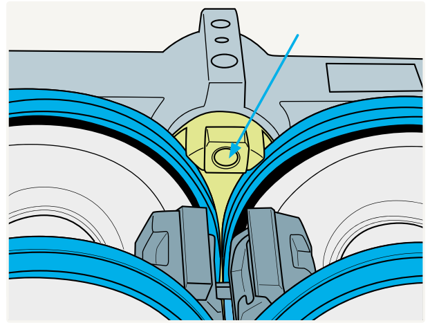
Fig. 25 – Positioning the magnetic bearing
