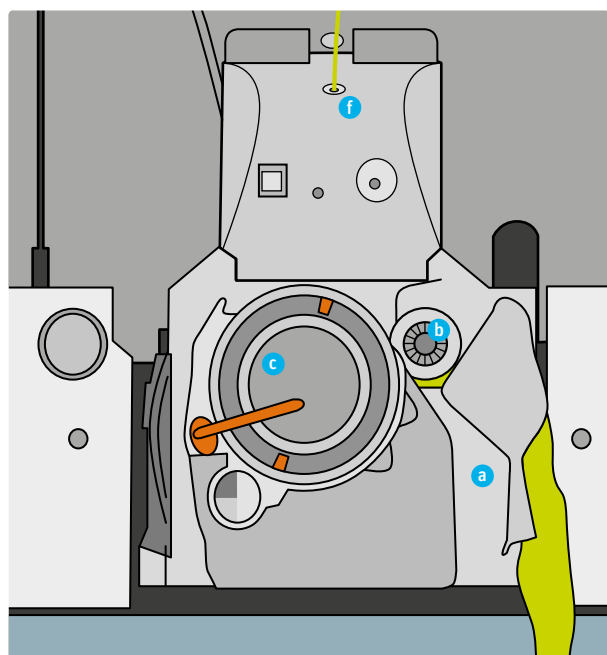
Fig. 8 – Front view of spinning box with opening roller and sliver intake
