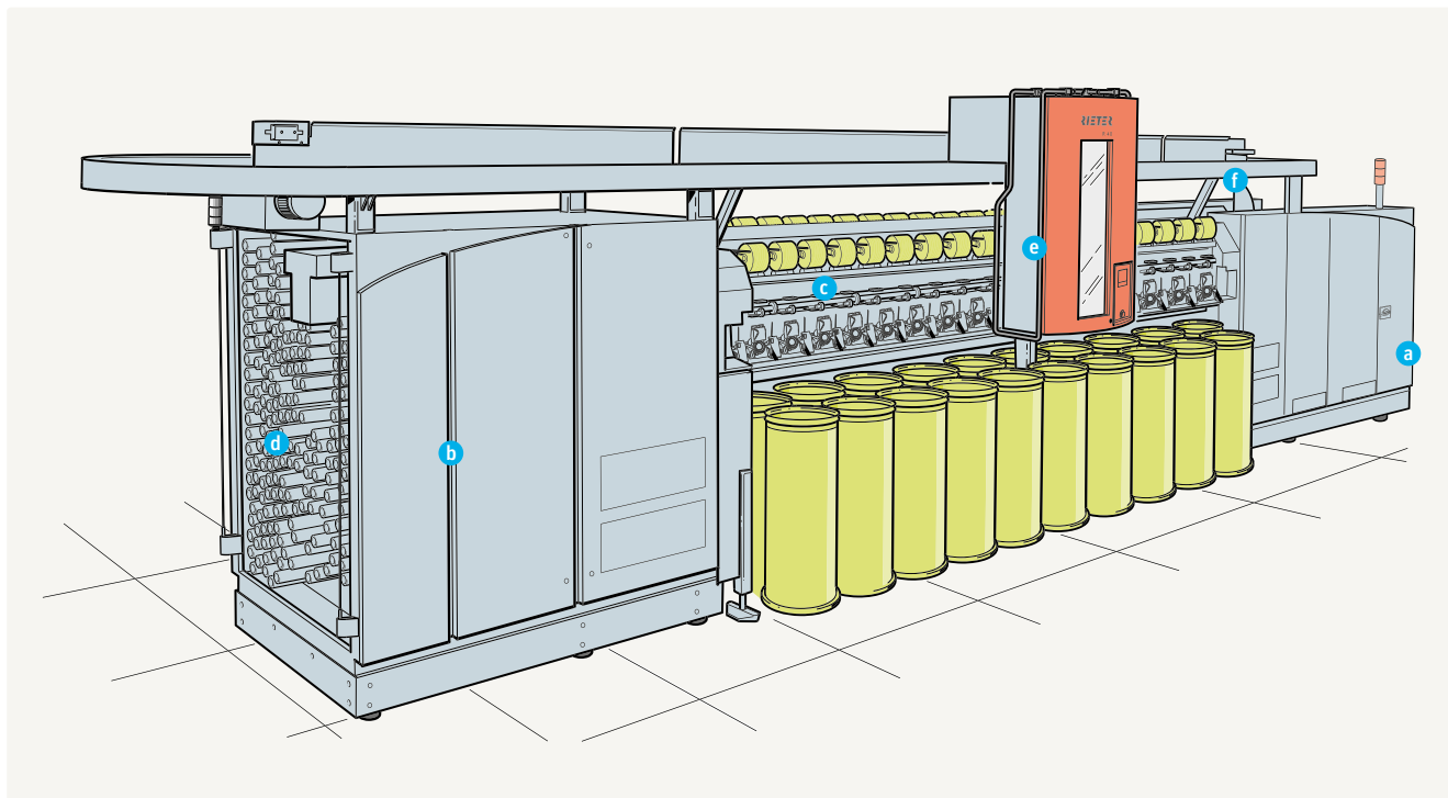
Fig. 6 – Structure of the rotor spinning machine
