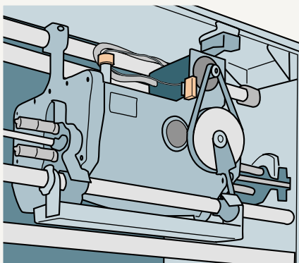
Fig. 35 – Gear for variable stroke displacement
