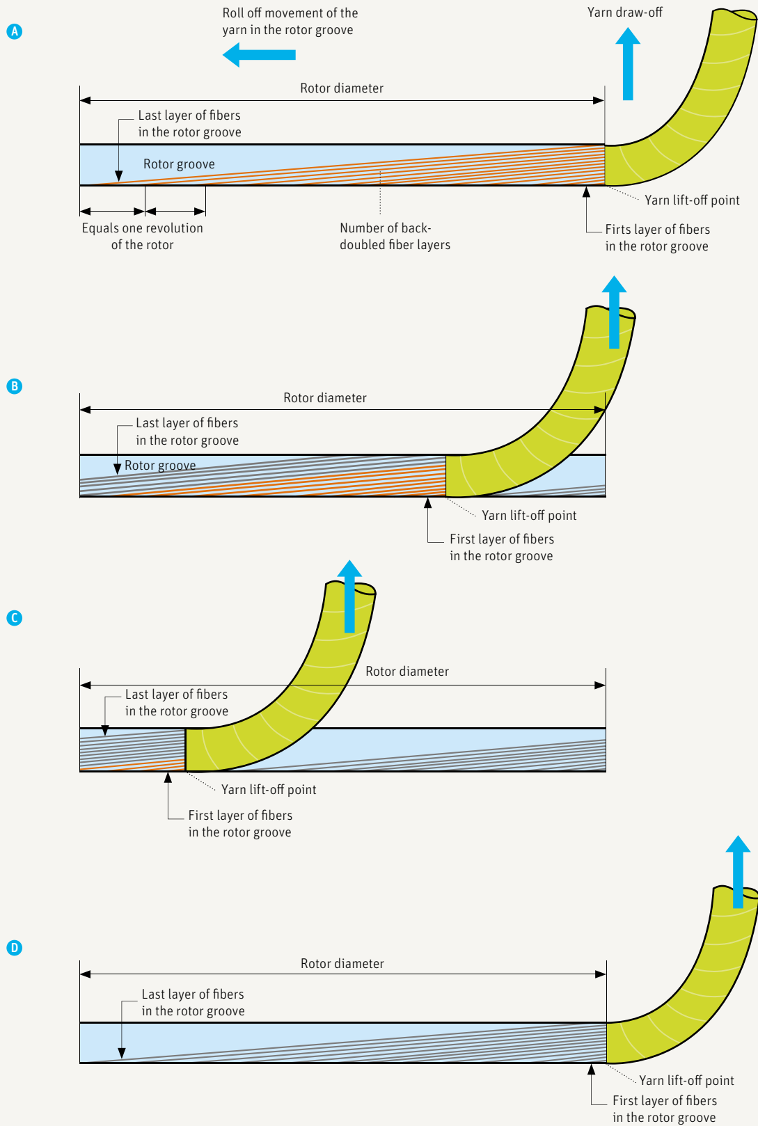
Fig. 93 – Illustration of the buildup of the fiber ring in the rotor groove by back-doubling and the corresponding position of the yarn lift-off point
