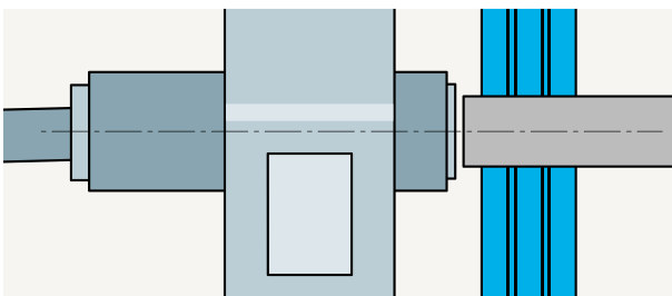
Fig. 28 – Axial rotor bearing with AERObearing
