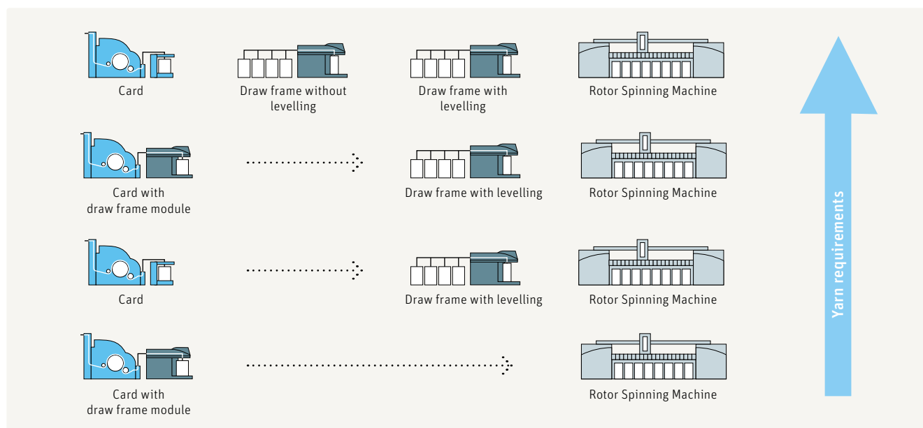
Fig. 71 – Rotor spinning systems with different sliver preparation depending on yarn quality requirements
