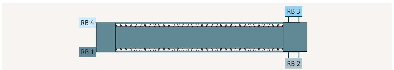
Fig. 53 – Rotor spinning machine with service stations for 4 robots
