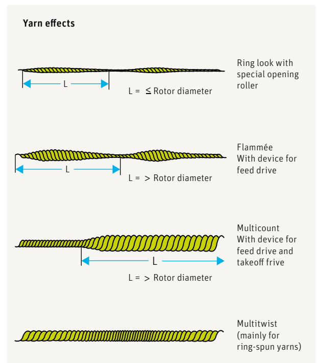
Fig. 88 – Yarn effects in rotor-spun and ring-spun yarns
