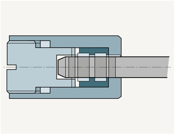
Fig. 24 – Axial rotor bearing with magnetic bearing
