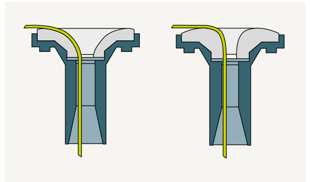
Fig. 84 – Ceramic draw-off nozzles with normal radius (left) and small radius (right)
