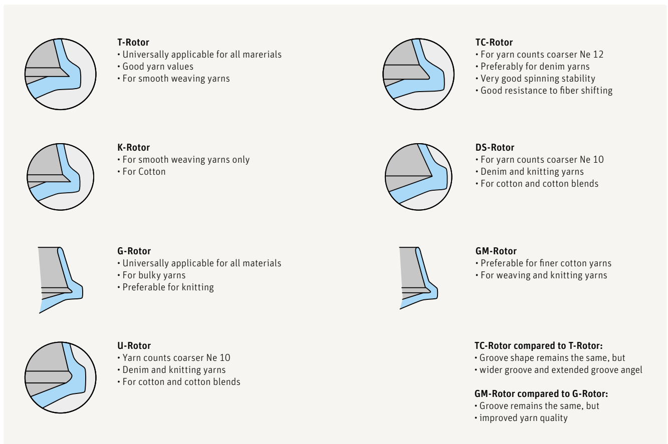
Fig. 77 – Configuration and properties of available rotor/groove shapes
