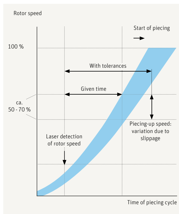
Fig. 59 – Automatic piecing during rotor acceleration
