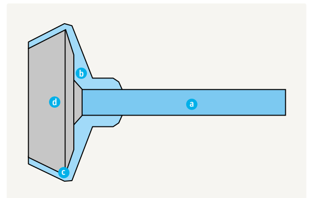
Fig. 75 – Structure and components of a spinning rotor: rotor shaft (a), rotor groove (c), rotor cup (b) and rotor wall (d)
