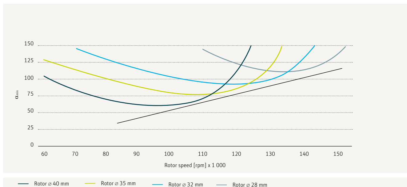
Fig. 19 – \alpha_{\min} values for different rotor diameters as a function of rotor speed (Source: ITV Denksendorf)
