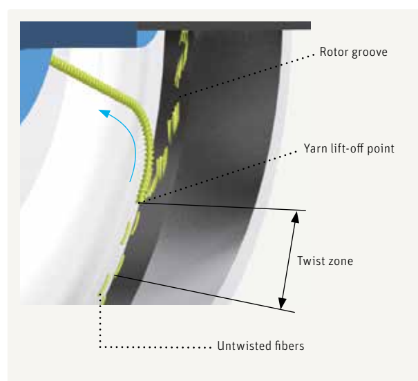
Fig. 94 – Inserting twist in the rotor groove
