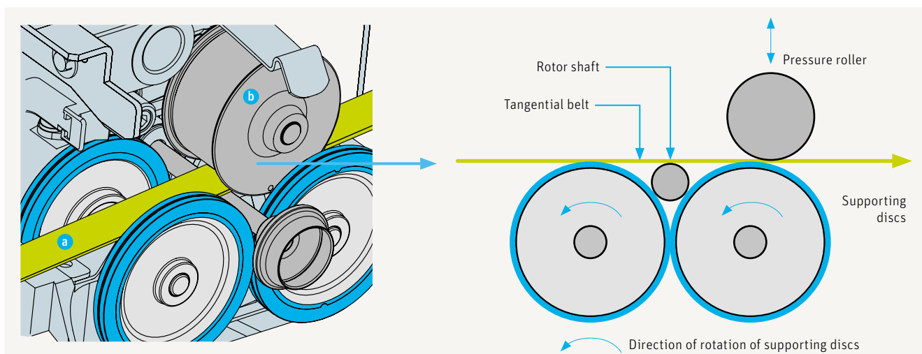
Fig. 23 – Support-disc bearing (Twindisc bearing) with pressure roller (b) for tangential belt (a)
