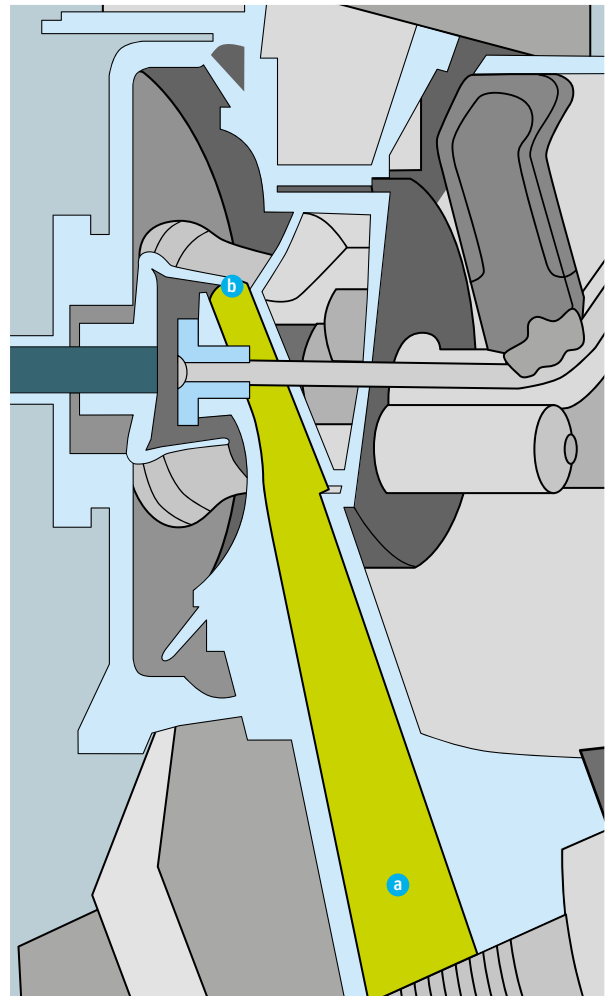
Fig. 14 – Cross-section through fiber guide channel (a) and spinning rotor (b)
