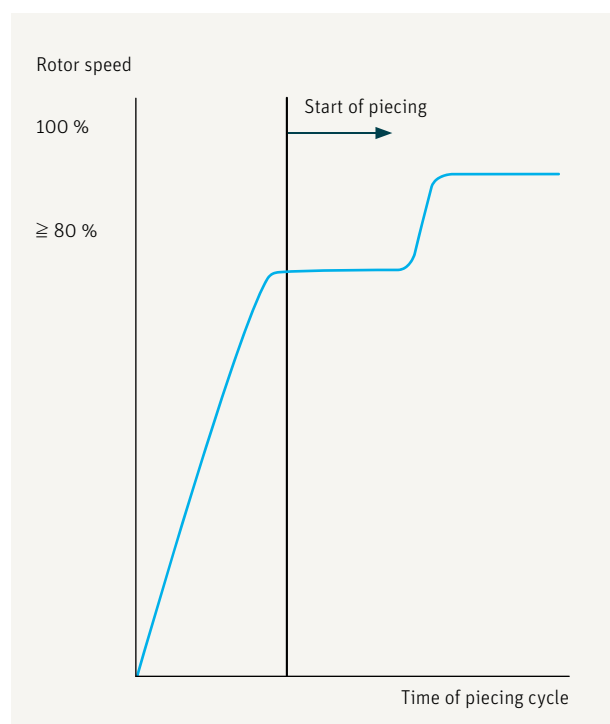
Fig. 58 – Automatic piecing at constant, high rotor speed
