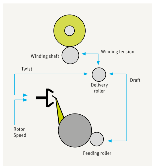
Fig. 39 – Infinitely adjustable inverter drives for draft, twist and winding tension
