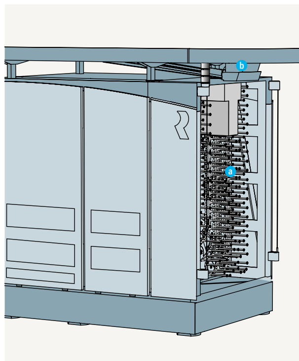
Fig. 62 – Empty tube magazine (a) with tube handling system (b) on the end frame of a rotor spinning machine
