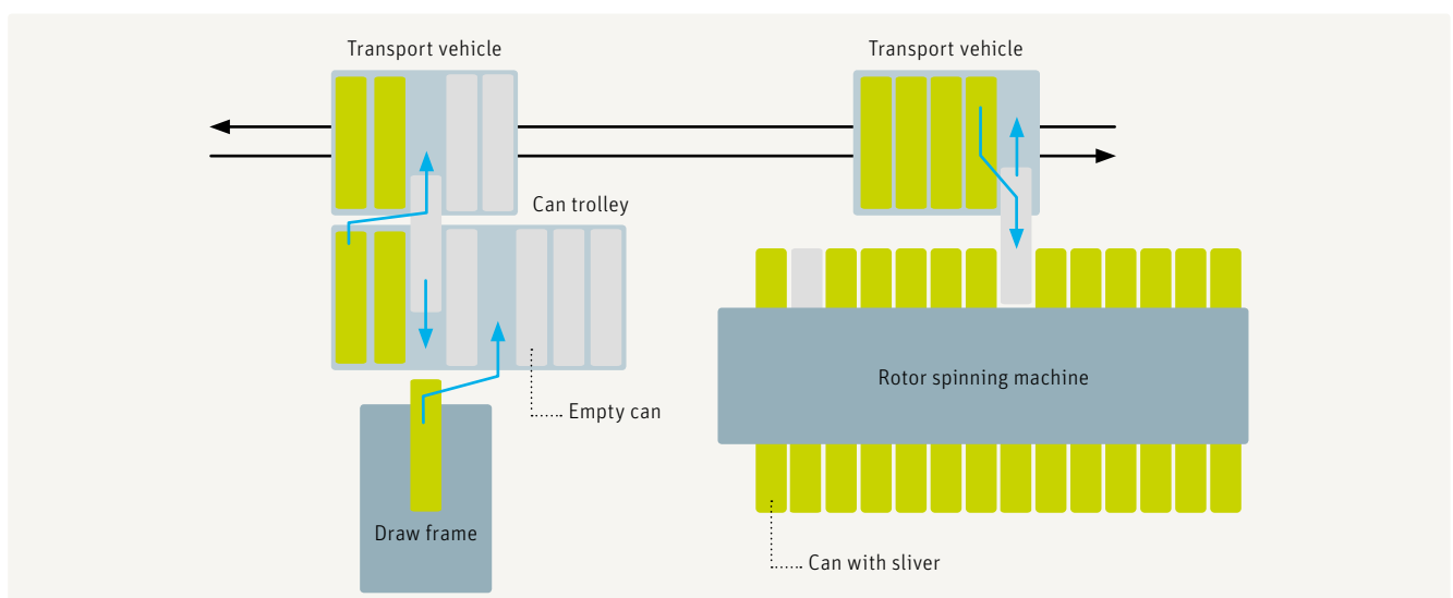
Fig. 64 – Concept for automatic can transport between draw frame and rotor spinning machine
