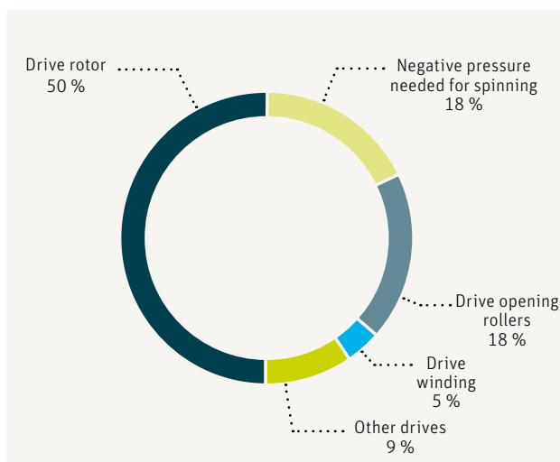
Fig. 38 – Breakdown of energy consumption for the various drives of a rotor spinning machine
