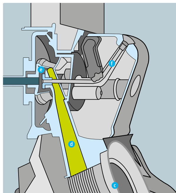
Fig. 9 – Spinning box cross-section
