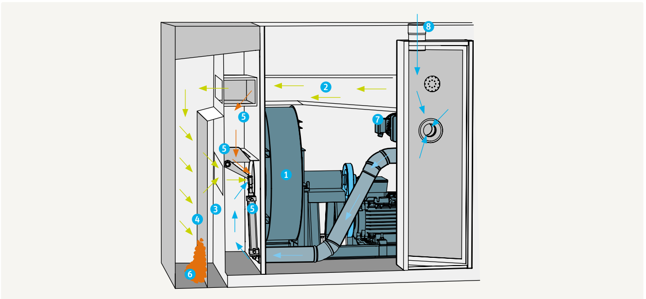
Fig. 42 – Negative pressure drive
