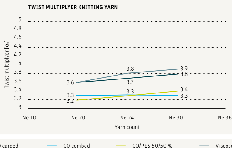
Fig. 92 – Twist multipliers customary in mill practice for rotor-spun knitting yarns
