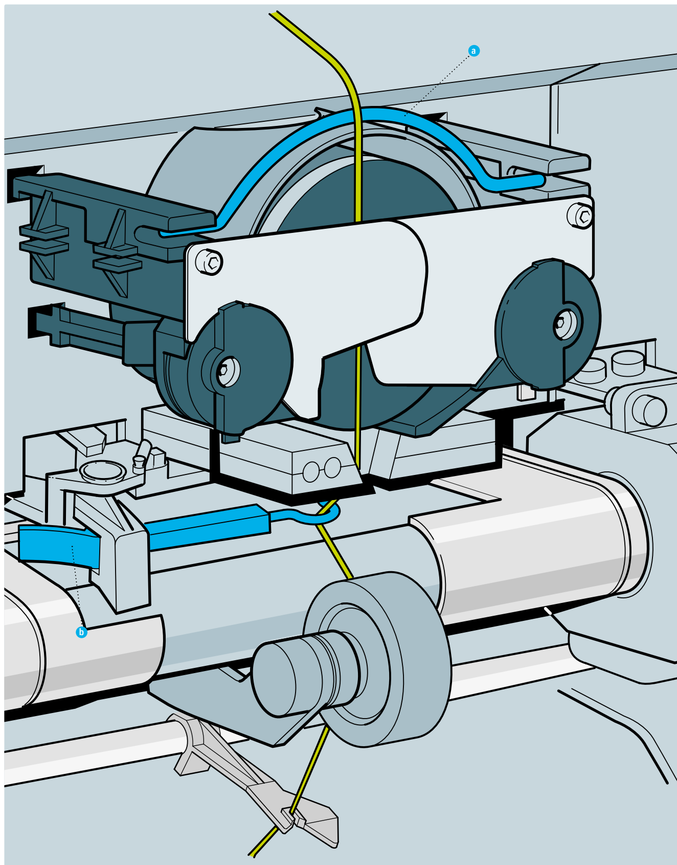
Fig. 32 – Compensation of winding tension with compensation bar (a) and yarn tension bar (b)
