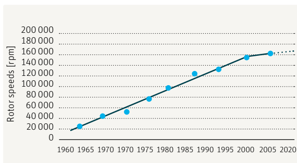
Fig. 1 – Development in achievable rotor speeds since the launch of the rotor spinning system
