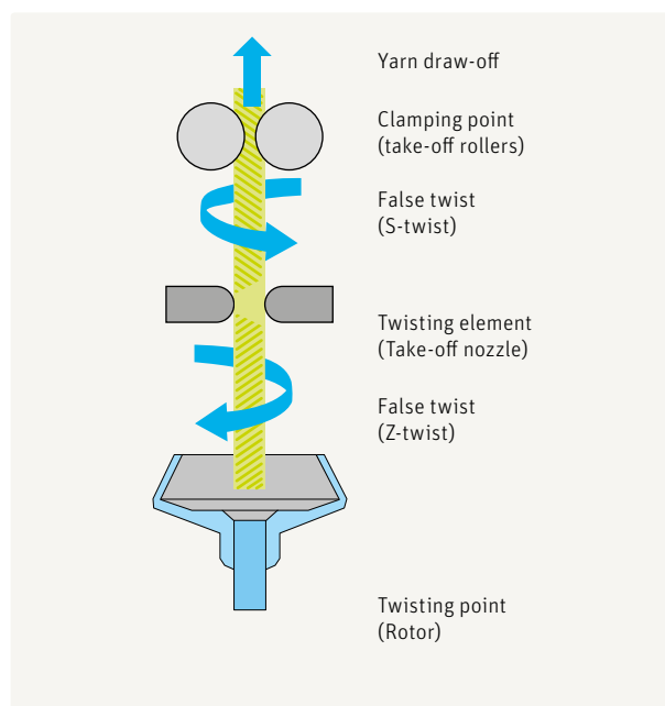
Fig. 97 – Imparting twist to the yarn: additional twist due to the false twist effect in the S and Z direction
