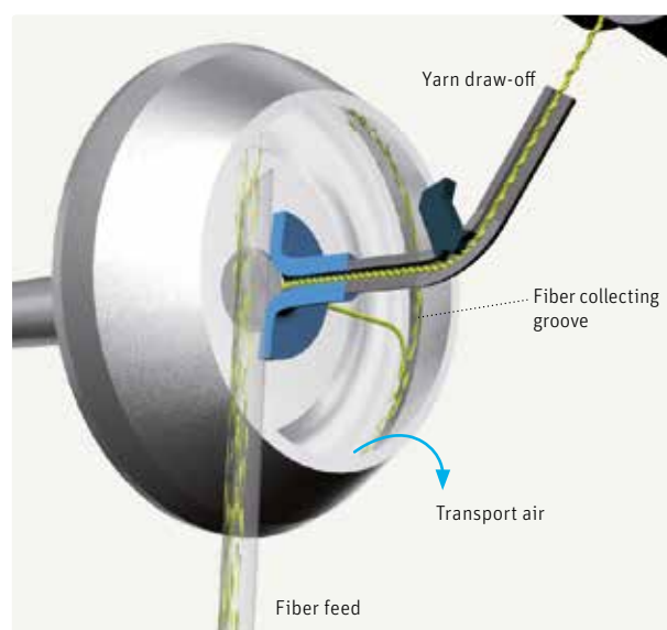
Fig. 16 – Tangential fiber feed into the rotor and fiber transport to the fiber collecting groove of the rotor
