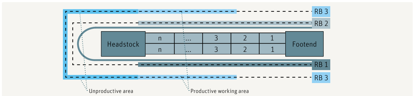
Fig. 50 – Travel strategy with 3 operating robots. One robot on each side of the machine, robot RB 3 serves each side alternately
