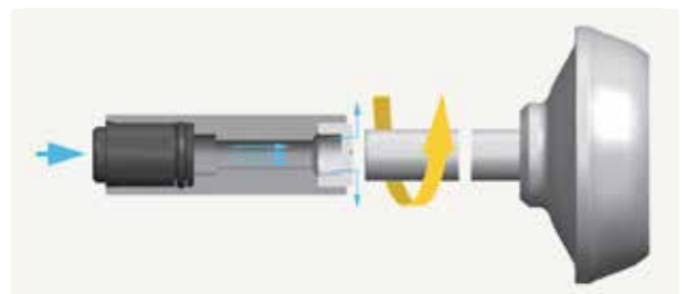
Fig. 29 – Airflow with the AERObearing; air pressure 6 bar
