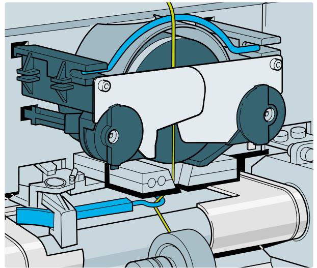
Fig. 37 – Waxing device with large wax blocks
