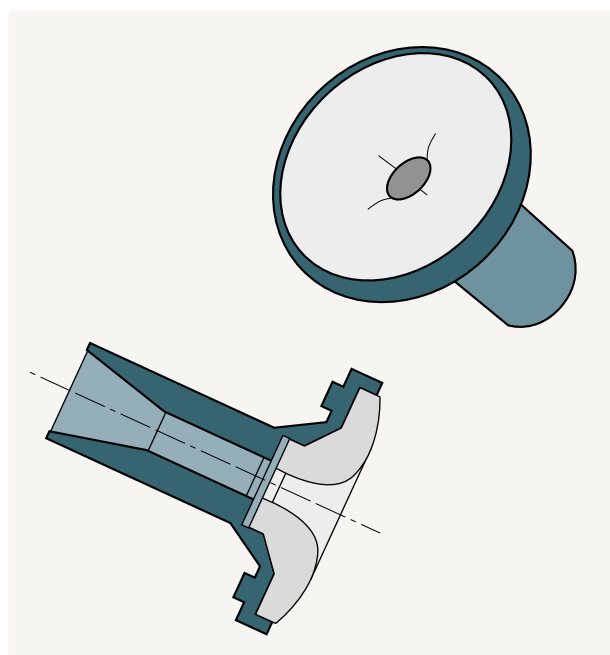
Fig. 78 – Draw-off nozzles with ceramic nozzle head and metal nozzle holder
