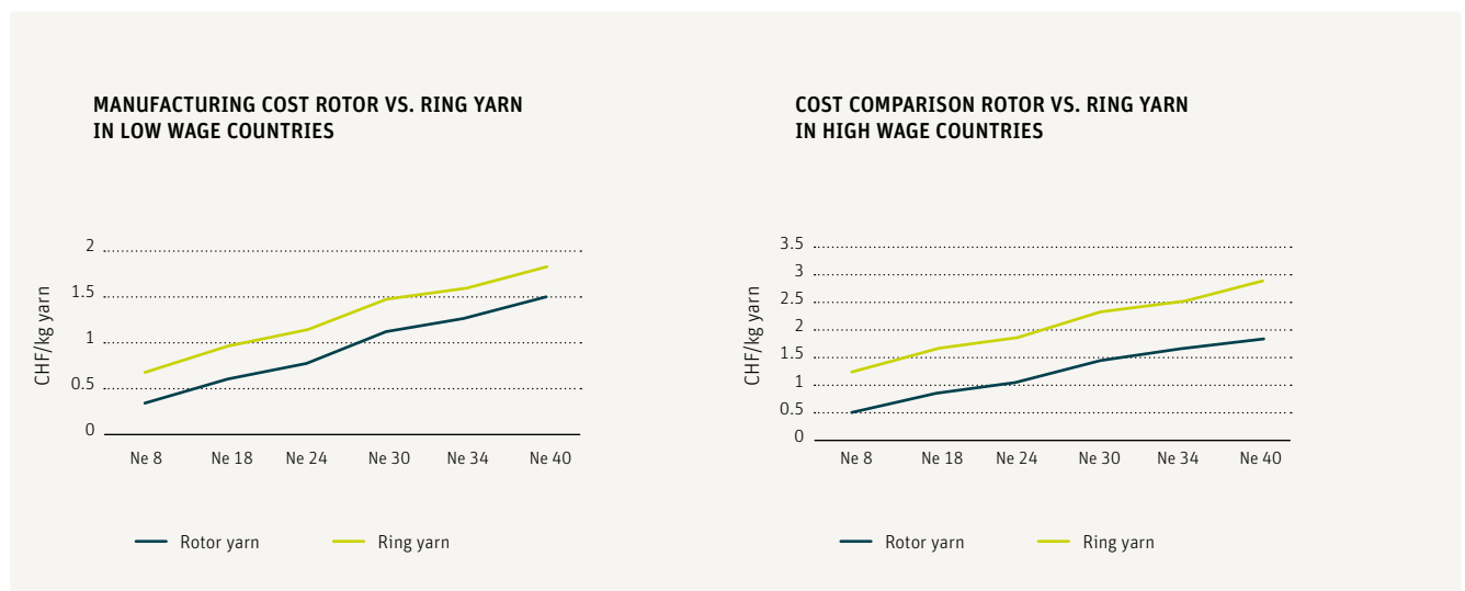
Fig. 100 – Comparison of manufacturing costs/kg of yarn for different yarn counts in low- and high-wage countries
