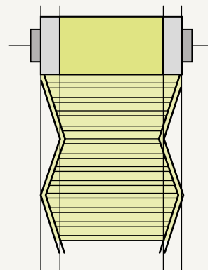
Fig. 36 – Variable stroke displacement
