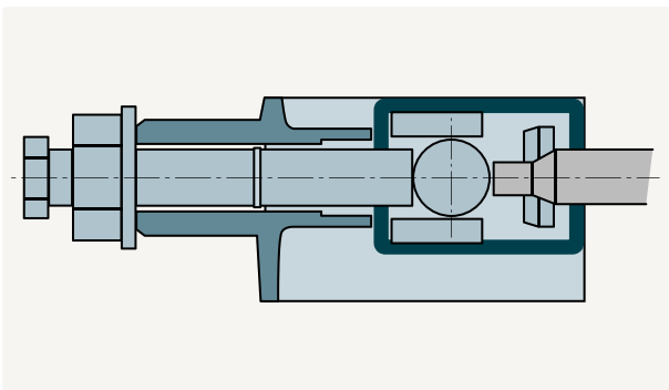
Fig. 26 – Axial rotor bearing with EC bearing
