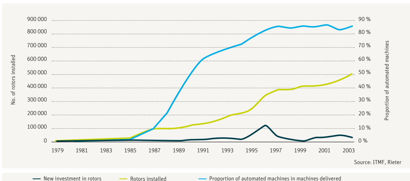
Fig. 3 – Number of rotors installed, showing the proportion of automated machines and new investment in rotors, using Turkey from 1979 to 2003 as an example
