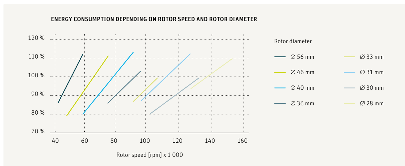
Fig. 101 – Energy consumption as a function of rotor speed and rotor diameter
