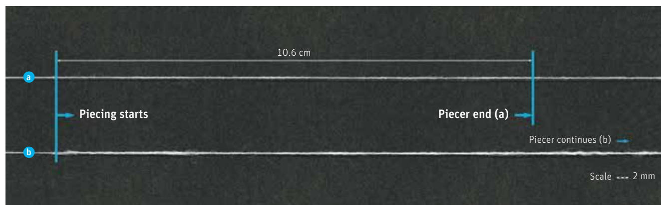
Fig. 54 – Piecing quality (Ne 30, Twist multiplier \alpha_e = 4.6 , 100 % cotton)
