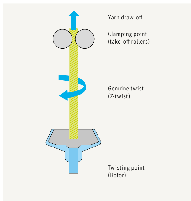
Fig. 96 – Imparting twist to the yarn: genuine twist in the Z direction
