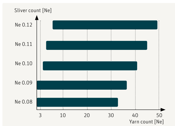
Fig. 89 – Maximum flexibility with drafts of up to 400-fold
