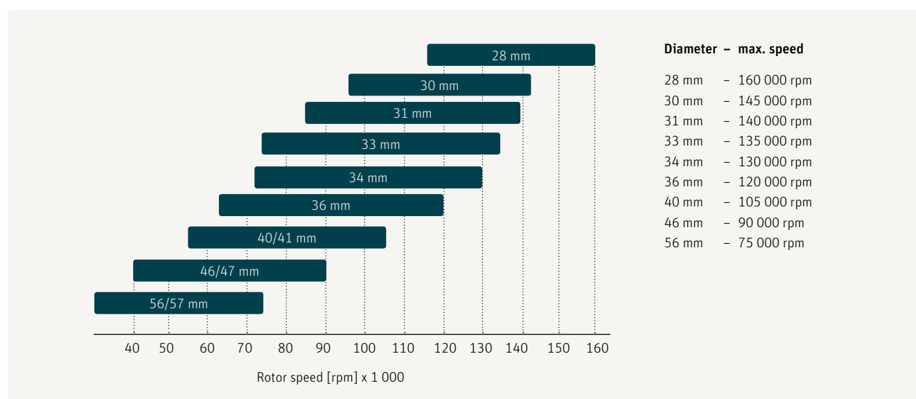
Fig. 76 – Speed range and maximum rotor speed as a function of rotor diameter (in practice rotor speeds are used up to about 5 - 8 % below the maximum)
