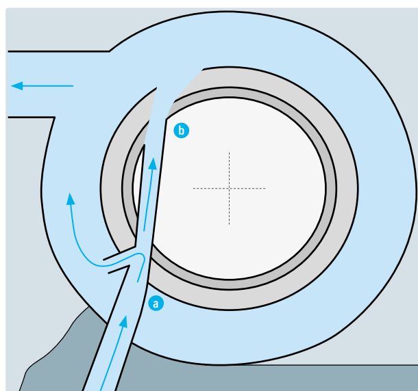
Fig. 15 – Fiber guide channel (a) with SPEEDpass (b)
