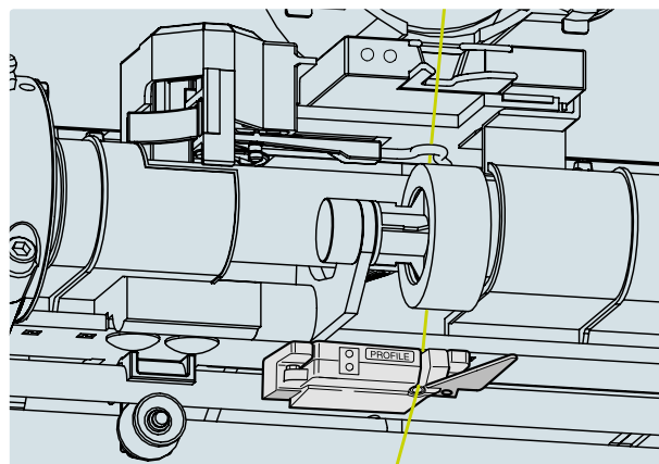
Fig. 46 – Barco Profile yarn clearer
