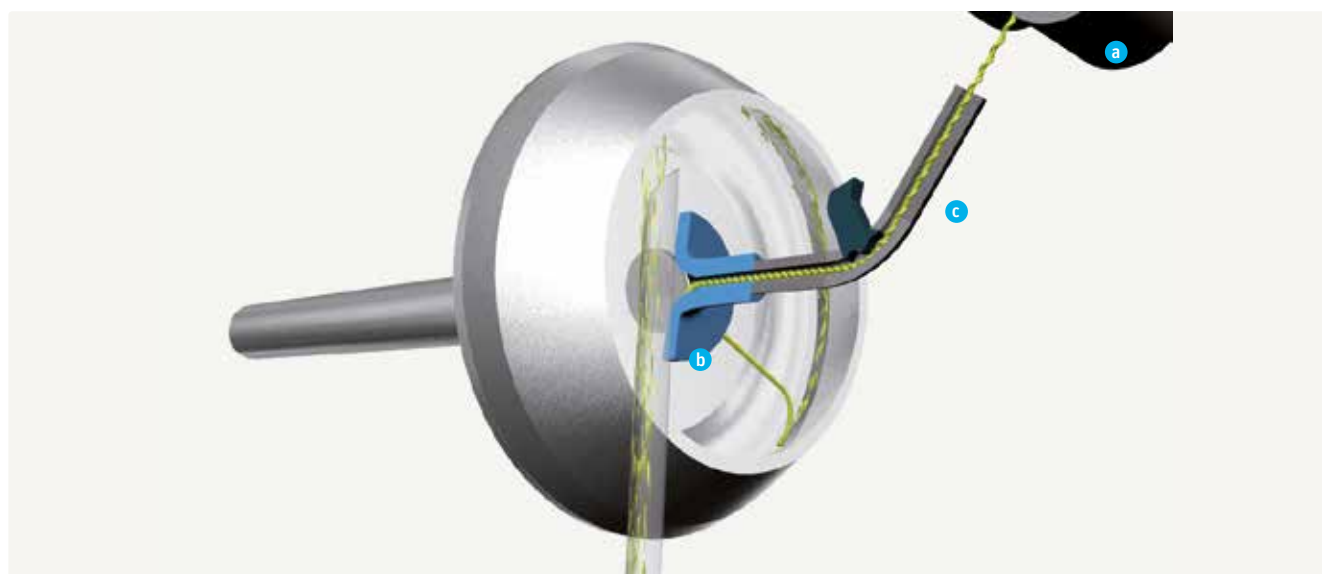
Fig. 30 – Yarn take-off with take-off rollers (a), draw-off nozzle (b) and yarn draw-off tube (c)
