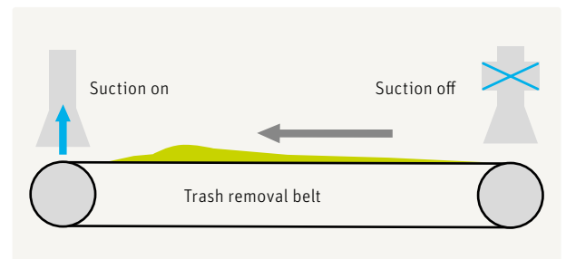
Fig. 41 – Trash removal belt with suction units
