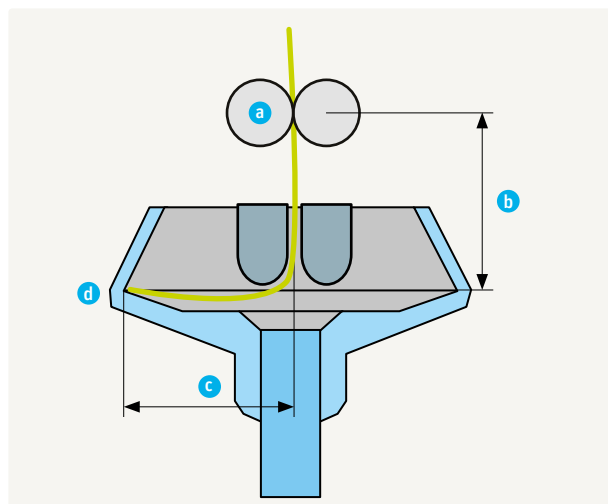
Fig. 95 –Inserting twist in the yarn
