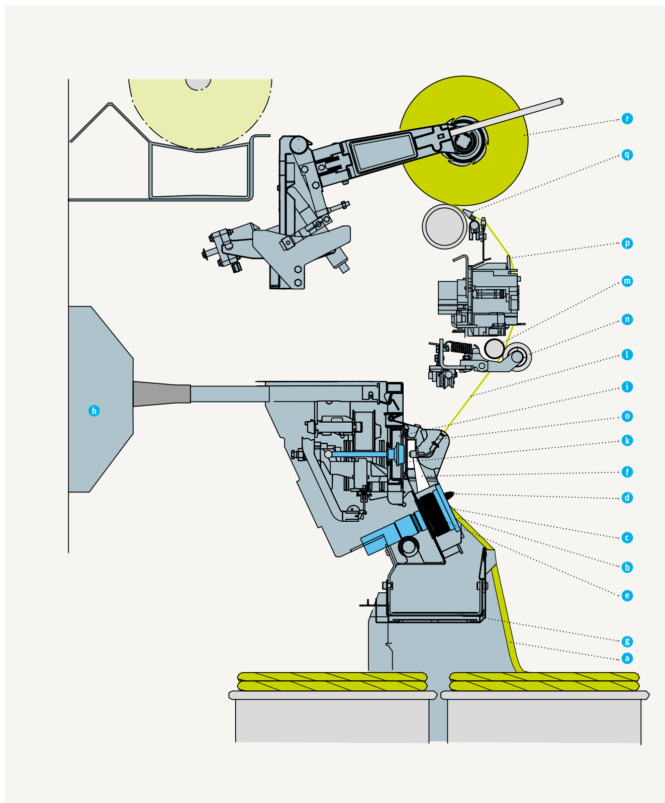
Fig. 7 – Path of the fibers from sliver feed into the spinning box to winding of the yarn onto cylindrical or conical cross-wound packages
