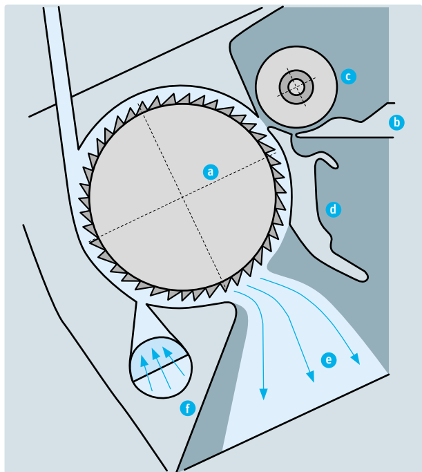
Fig. 10 – Opening roller housing with opening roller (a), sliver intake (b+c), fiber beard support (d), trash removal (e) and adjustable bypass (f)
