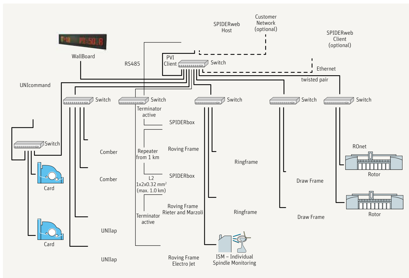
Fig. 47 – System diagram of production monitoring; central computer with peripherals and connected production machines
