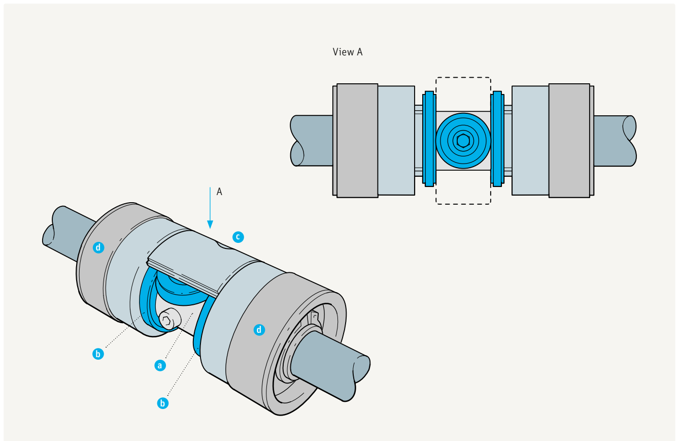
Fig. 33 – Three-part winding cylinder with powered middle section (a), two powered side sections (b), wheel and disc differential gear (c) and friction coatings (d) for driving the package
