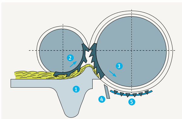
Fig. 95 – Conventional feed device
