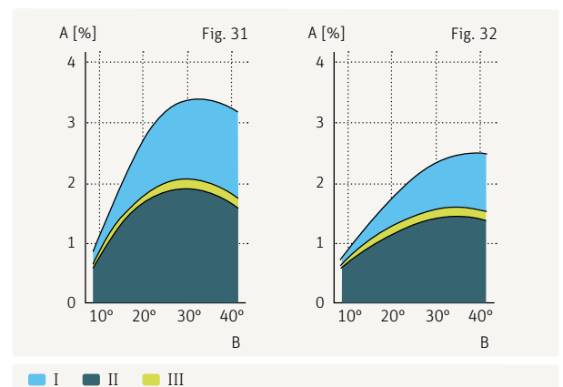
Fig. 31 – Dependence of waste elimination: (A, %) on the setting angle of the grid bars relative to the beater (B in degrees). I, fiber content; II, trash content; III, filter drum loss (Beater rotation speed: 740 rpm).
