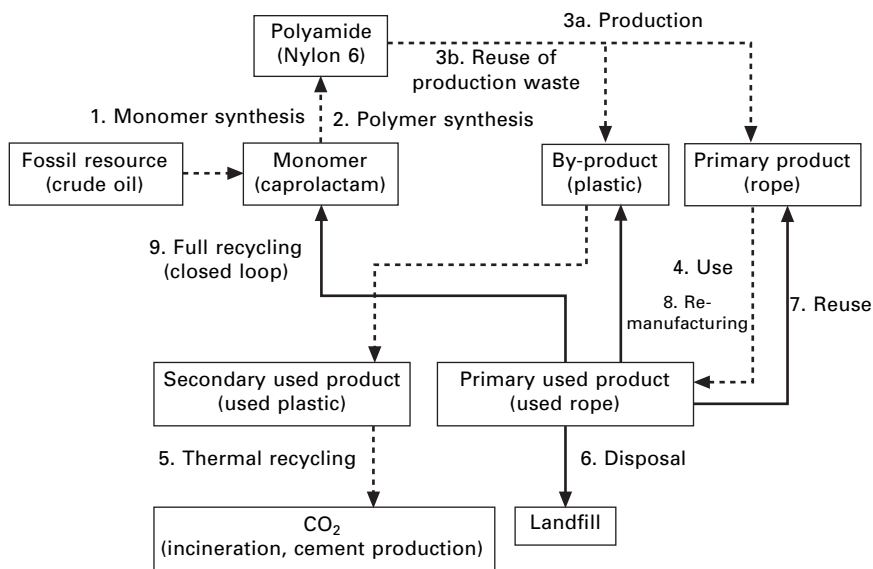
4.24 Options for material flow of nylon recycling in Switzerland. Some options require international transportation for economic reasons such as productivity of a plant (see also Fig 4.23).
