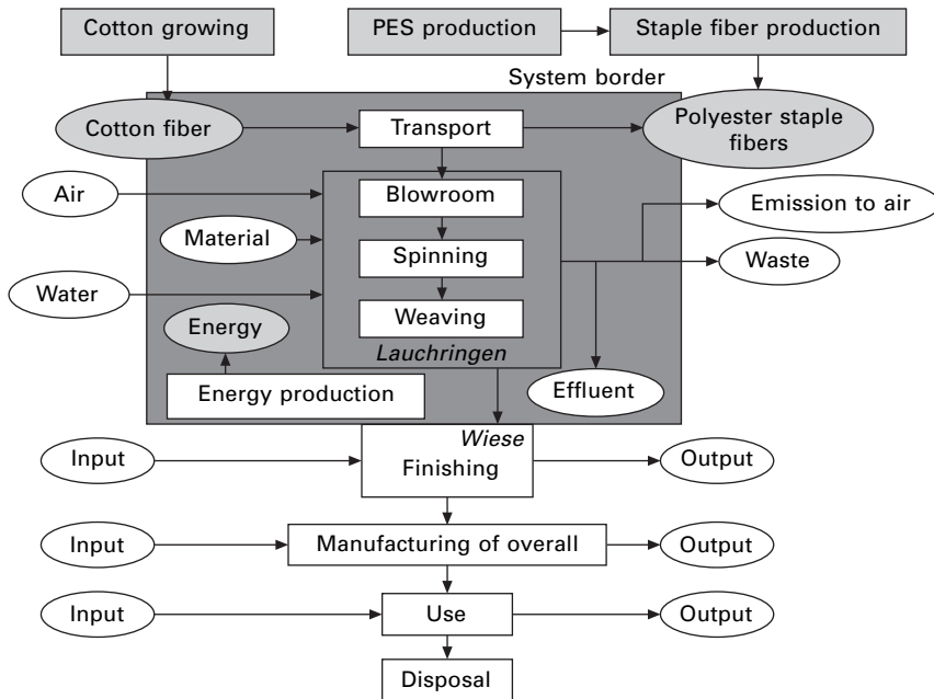
4.8 System modeling of case study D. The main system is underlain in dark gray, the additional flotation and the additional energy supply in light gray.
