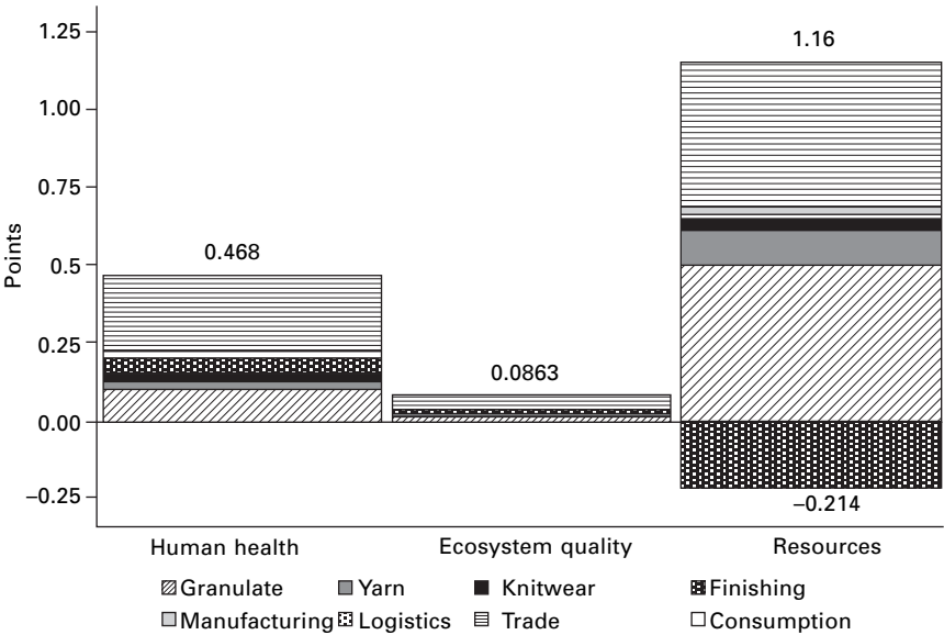
4.49 Aggregated LCA results for the production of the PES T-shirt (same system as for Fig. 4.48) in EcolIndicator 99.
