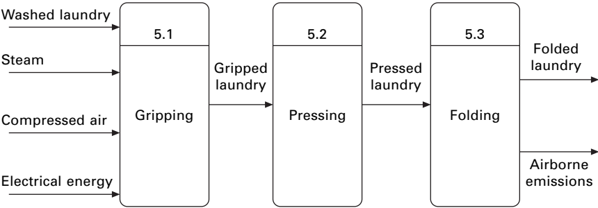
4.22 Detailed sub-processes and material flows for the mangling process 5 (see Table 4.12) in case study F.
