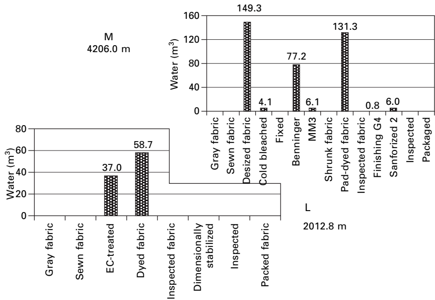
4.43 Water consumption of the two fabrics M and L in finishing (case study E).
