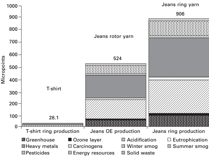
4.33 ILCA results (method EcoIndicator 95) for 1 m 2 of a knitted product (T-shirt) and two woven products (jeans), produced by two different technologies. As the energy life cycle is included in the system, the low impact of the knitted fabric is achieved by both the knitting technology and hydropower energy (production on the plant).
