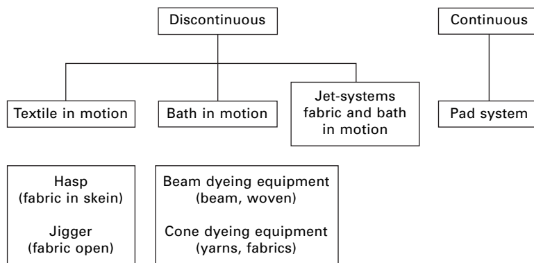
3.31 Variations in finishing technology with different processing equipment (discontinuous, batch) and different fabric configurations (open and skein).
