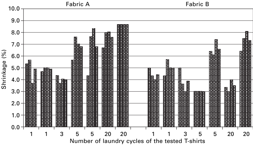
3.49 Dimensional stability of two knit fabric types after one, three, five and 20 laundry cycles (with repetitions for five and 20 cycles). Fabric B shows very inconsistent quality with five and 20 cycles.
