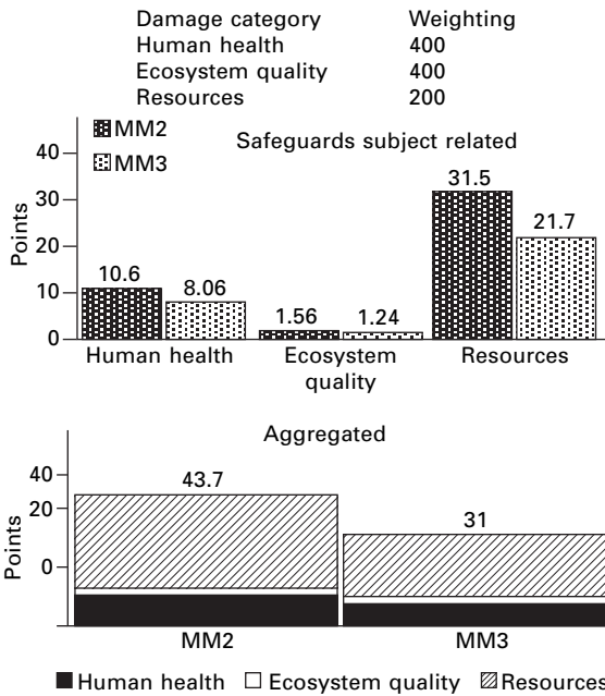
4.47 Detailed comparison of two pre-treatment technologies applied for fabric M (case study E) with method EcoIndicator 99 (subject related and aggregated). The weighting factors are given at the top. One point (Pt) relates to 10^{-3} average annual impact of a European consumer.
