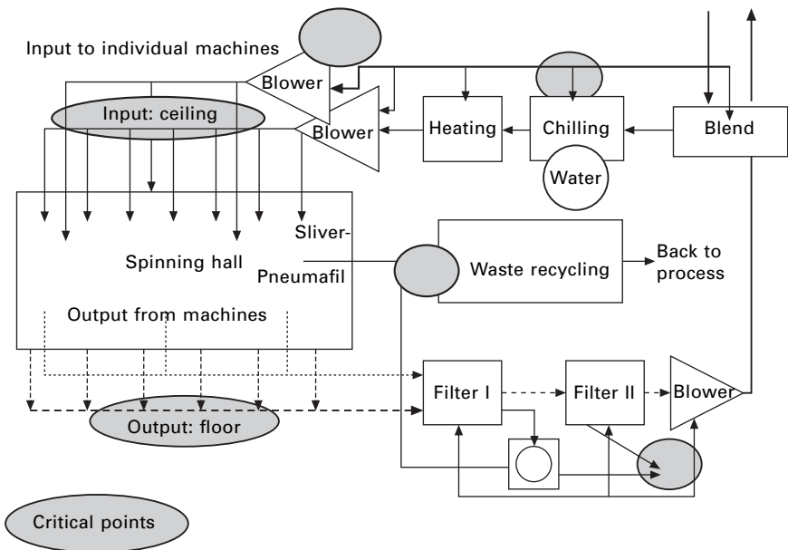
3.45 BAT in air conditioning: critical points (gray areas) are input and output positions, a floating chilling (following the outside temperature), and appropriate cleaning of filters.
