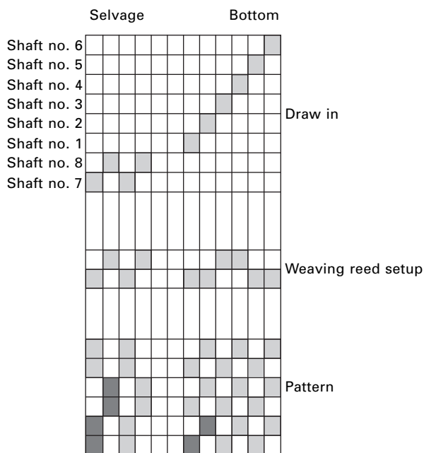
3.25 Setup and weaving reed for a canvas fabric (weave type 1/1). The selvage is formed in a different weave and color.
