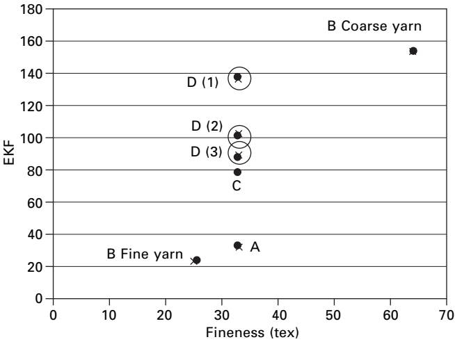
4.80 EKF for spinning for individual products from companies A, B and D (three different products).
