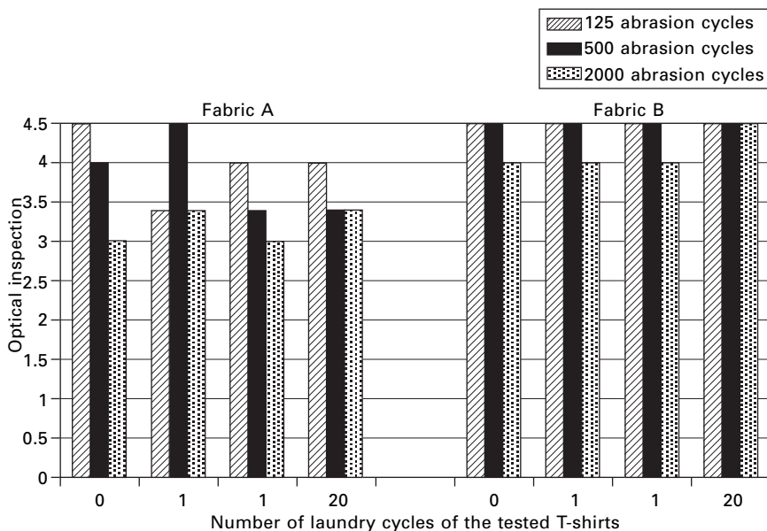
3.51 Pilling of two knit fabrics after one and 20 laundry cycles, equivalent to abrasion cycles.
