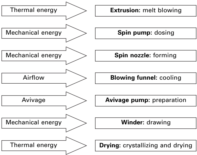
3.35 Melt spinning processes with inputs, equipment and processes.
