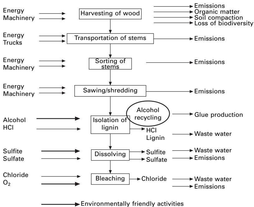
2.36 Process overview of pulp production for viscose generation.
