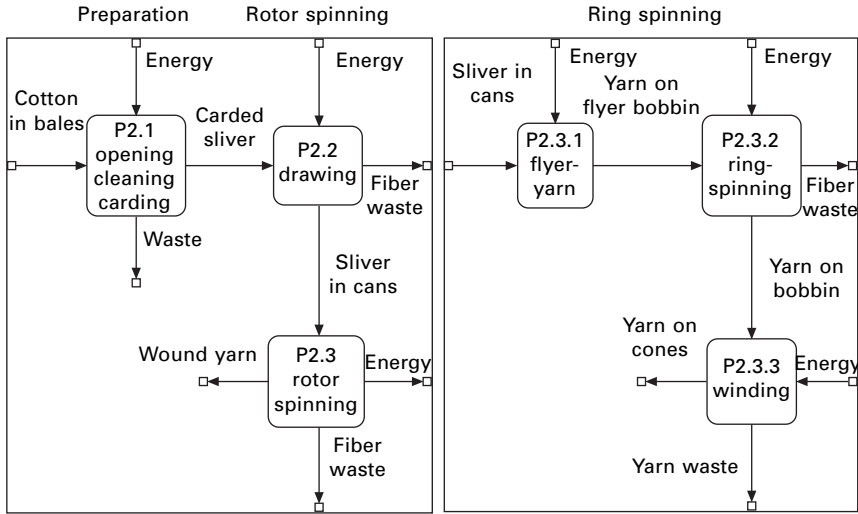
4.16 Spinning processes and material flows of two different spinning technologies (studies B and C).
