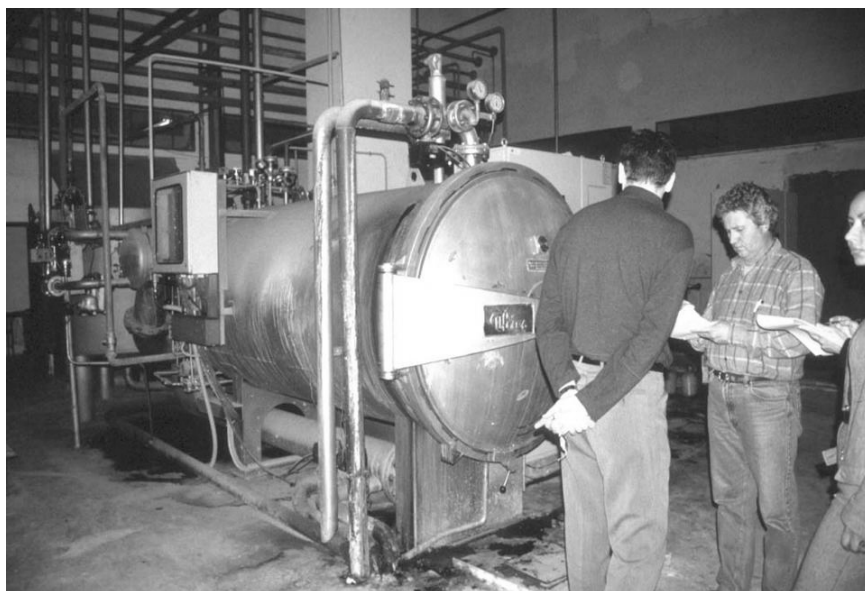
2.58 Jet dyeing machine for dyeing processes in exhaustion technology.
