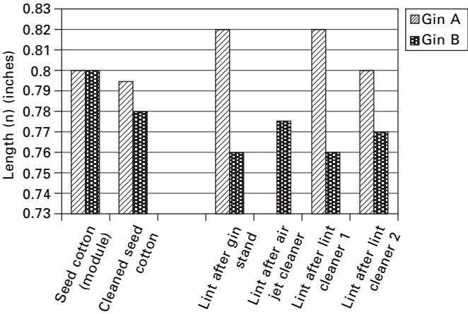
3.8 Fiber length (n) of cotton processed in two different gins. Gin B, working with high productivity, produces somewhat shorter fibers than Gin A, operating with a lower productivity.
