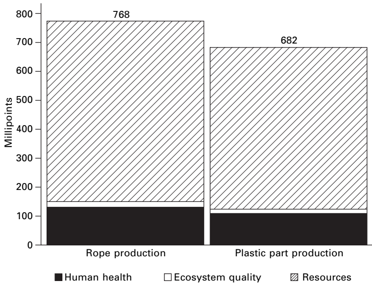
4.60 LCA results for rope production and plastic part production from PA 6 (case study H).
