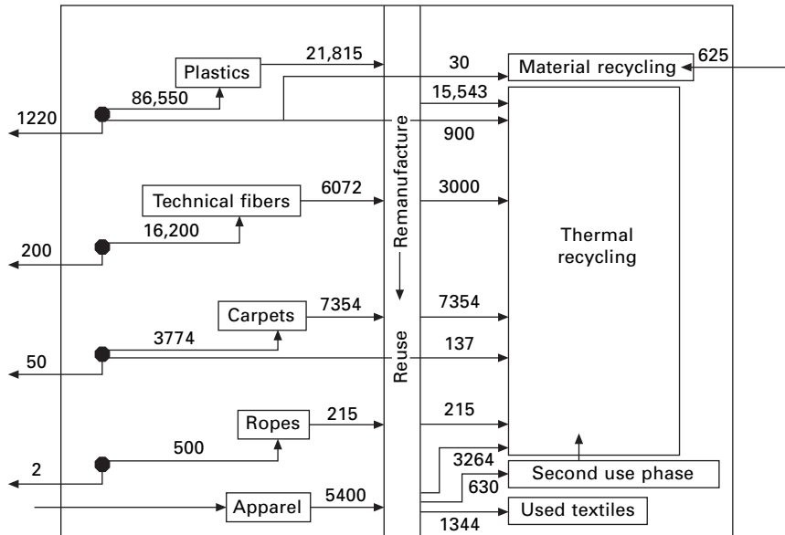
2.66 Product-related material flows (tons) of polyamides for recycling and reuse (Swiss case study).
