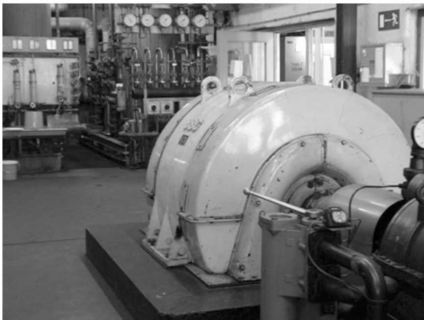
3.48 Steam production for finishing in a diesel generator. The choice of the prime energy source determines the environmental impact, which is considerable with diesel compared to gas, but better than for crude oil.
