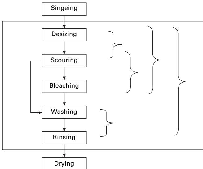
3.29 Variations in pre-treatment of cotton fabrics. The brackets indicate the processes which can be combined. Quality aspects have to be considered because substances remaining from the preceding process may disturb the following chemical reactions and produce inferior quality. Washing and rinsing remove disturbing chemicals but are more costly and time consuming.
