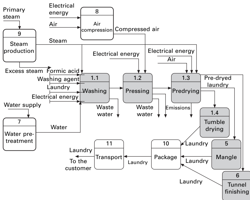
4.20 Laundry processes and material flows for the professional laundry process of case study F. Processes 1.1, 1.2, 1.3, 1.4, 5 and 6 are primary processes (gray). Steam production, air compression and water pre-treatment are auxiliary processes included in the system.
