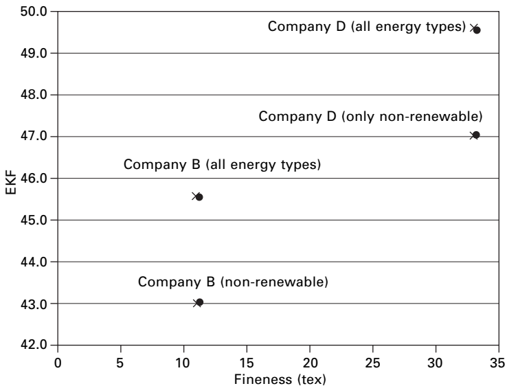
4.78 EKF of the spinning processes: calculation based on non-renewable energy.
