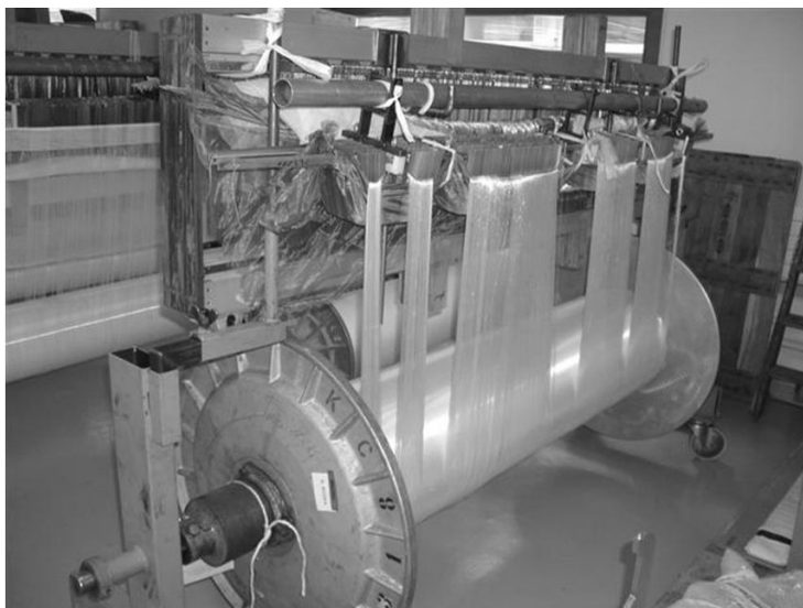
3.46 Threaded warp beam. Automated threading requires a few hours while manual threading takes three to four days' labor.
