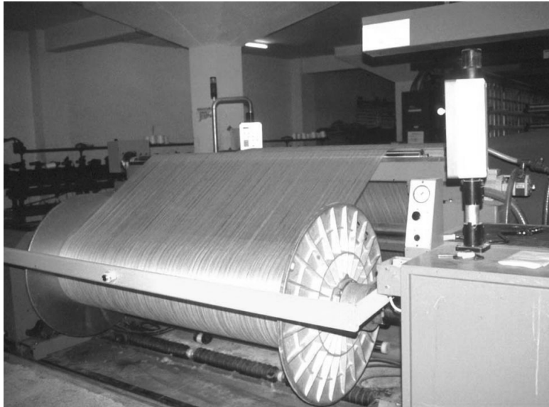
2.49 Sectional beaming and assembling.
