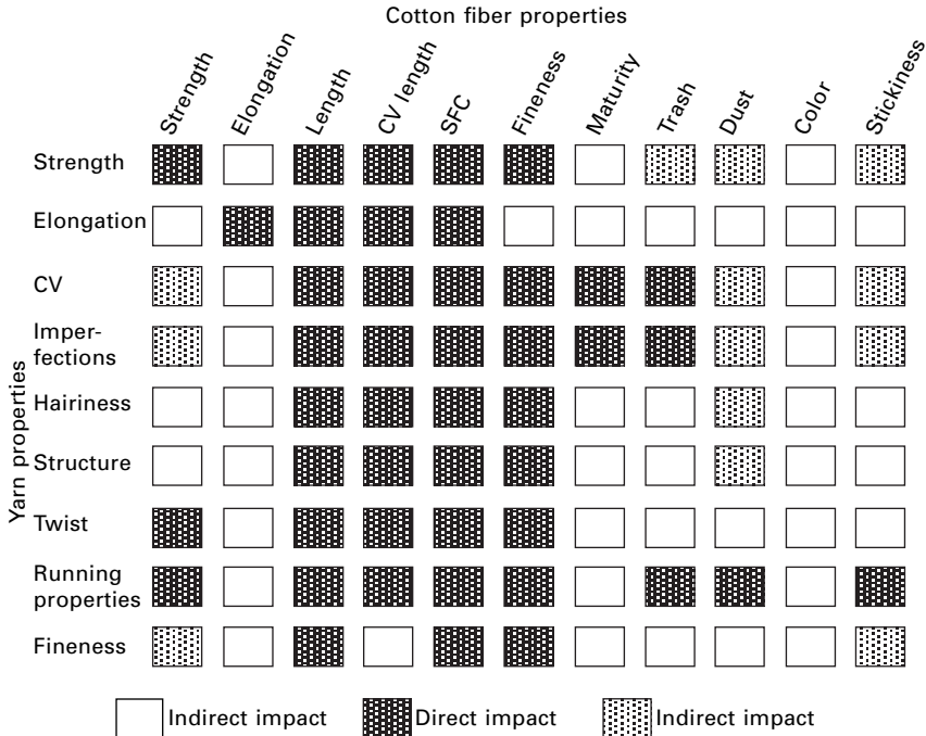
3.14 Correlation matrix of cotton fiber properties and yarn properties. CV = uniformity, SFC = short fiber content.
