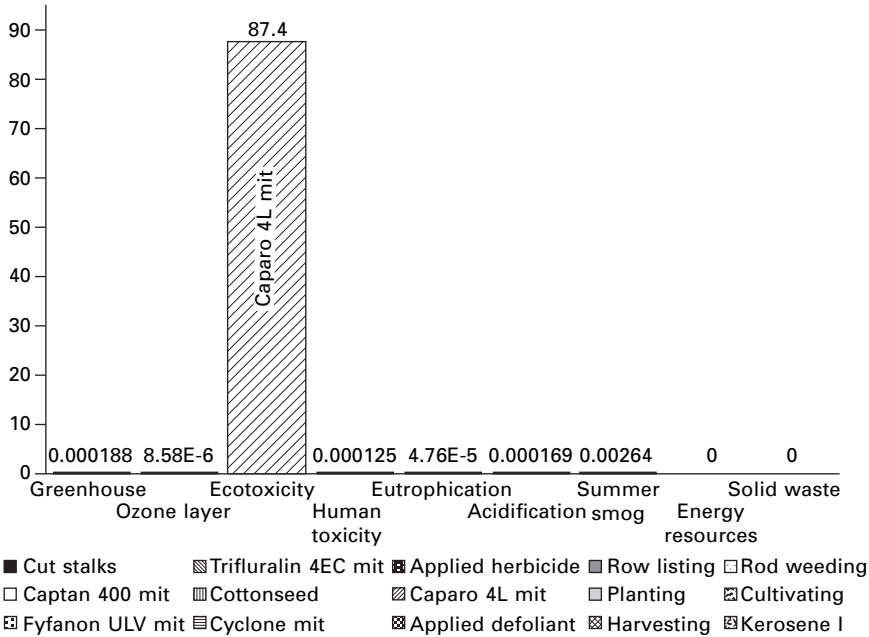
4.26 LCA results (in millipoints) of dryland cotton (method CML) of case study A.
