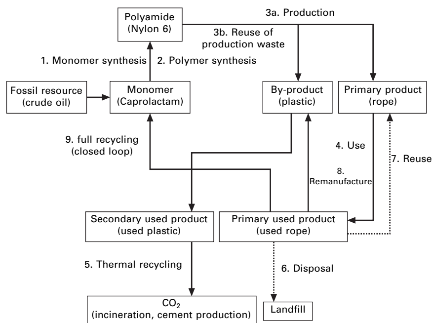
2.67 Recycling options for Nylon (PA 6.6) include full recycling, remanufacture, reuse, thermal recycling and disposal.
