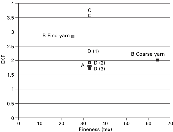
4.81 EKF for spinning for products from companies A, B and D: calculation based on CO 2 emissions.
