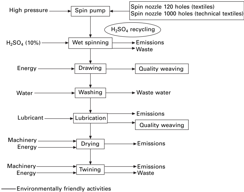
2.39 Viscose production processes: wet spinning.
