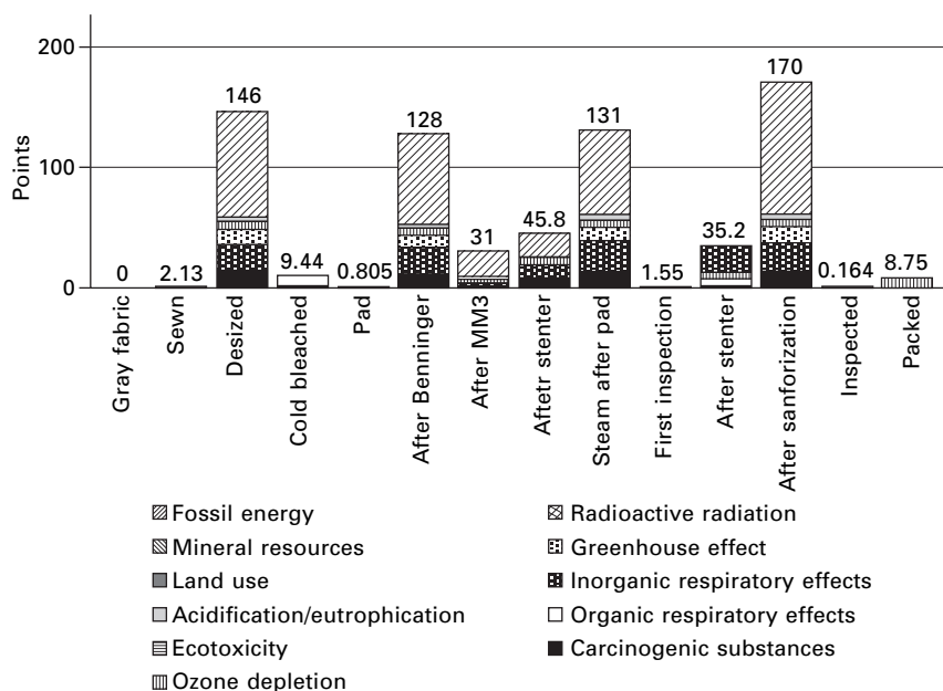
4.45 LCA results of the finishing processes for fabric M (case study D).
