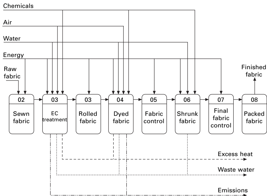
4.17 Finishing processes and material flows for fabric L in case study E.
