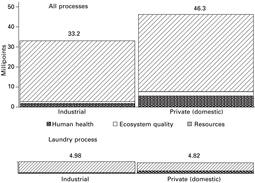
4.51 LCA results for professional and private laundry (including washing) and washing processes (case study F).
