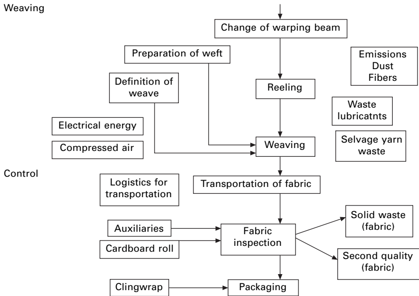
2.53 Processes and material flows in the weaving department and in control.
