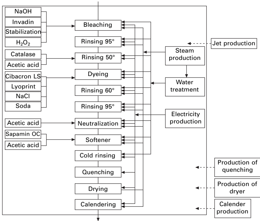
2.55 Finishing processes with inputs in the pre-treatment, dyeing and finishing sections for a cotton fabric (source: Zwicker 1997).
