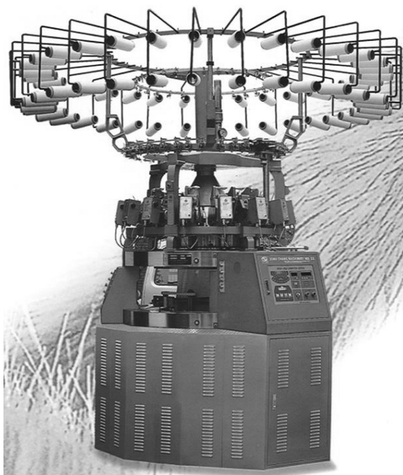
2.54 Circular knitting technology with 92 knitting systems.
