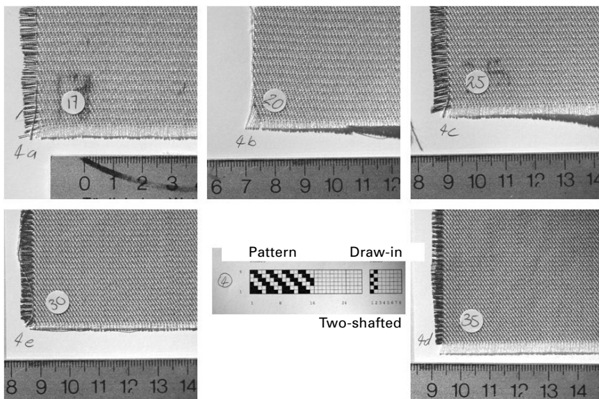
3.21 Traditional twill fabric (denim) with two colors and variations in weft density: 17, 20, 25, 30 and 35 counts per cm. The frame setup is based on a two-shaft draw-in.
