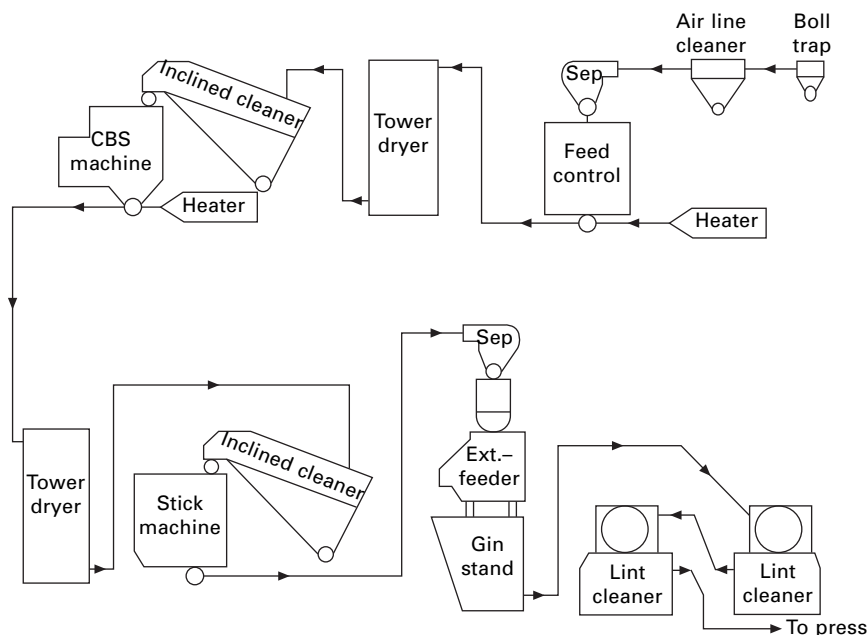
2.27 Schematic view of ginning processes with new CBS machinery for bur extraction. The second lint cleaner may be bypassed.
