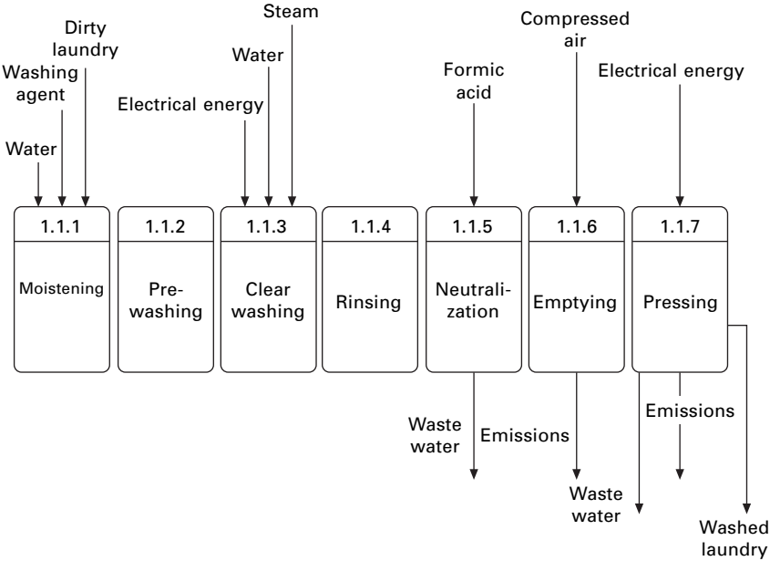
4.21 Detailed sub-processes and material flows for the washing process 1.1 (see Table 4.12) in case study F.
