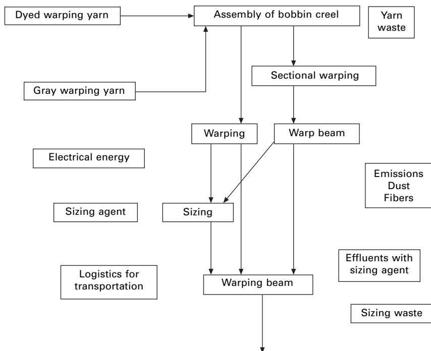
2.47 Weaving preparation processes.
