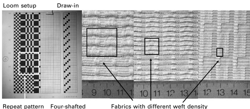
3.22 Structural design pattern with canvas weave and one color. The three frames show three weft densities.
