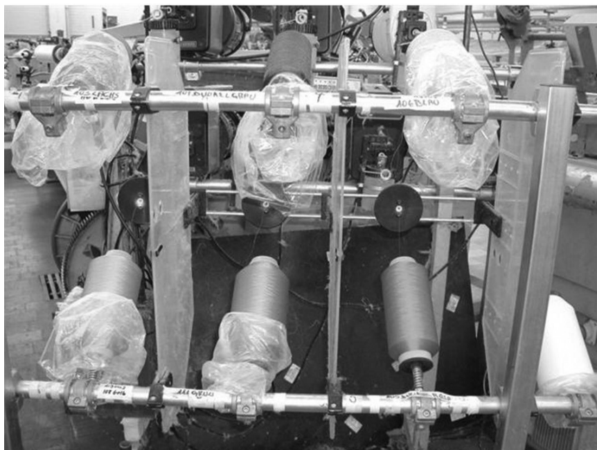
2.52 Insertion of different colored weft yarns.
