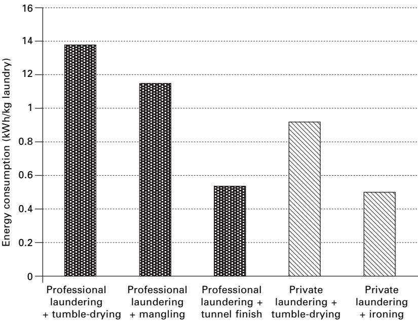
4.52 Energy consumption of laundry processes (case study F) (source: Pulli 1997, Affolter and Steiner 2002).
