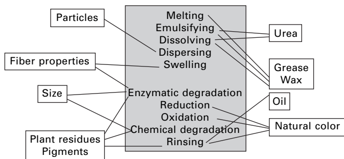
3.27 Principles of pre-treatment: the naturally existing impurities like particles, wax, etc., in natural fibers (white) are removed by means of different chemical–physical reaction types (center panel). Often several reaction types are available. Process auxiliaries like size and oils can be degraded with the same mechanisms. Fiber properties can be improved with swelling (mercerizing) and enzymatic treatment (removal of seed coat fragments).
