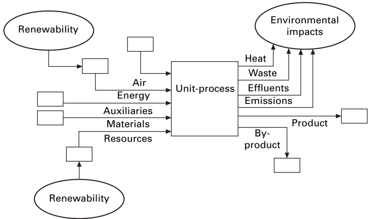
4.12 Scheme for input-output analysis defined for a (central) unit process. The unit process is applied along all chains of the investigated product life cycles.
