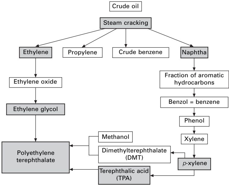
3.34 The two production lines for TPA, the monomer base for polyester.
