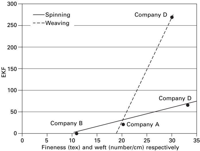
4.77 EKF of the spinning and weaving processes. The weighting factors for the individual energy sources were taken according to E95.
