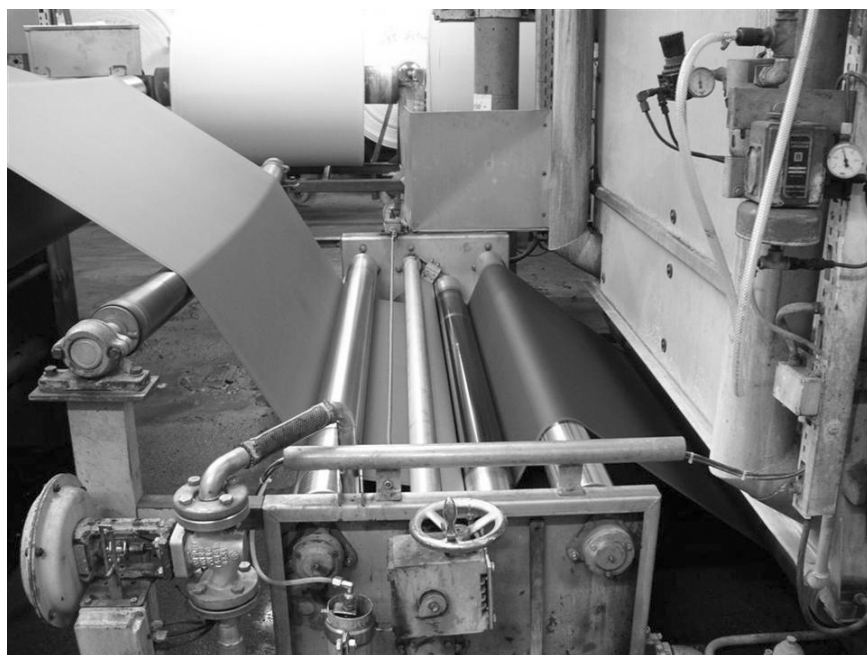
3.32 Pad system for wet processes. The fabric (left side) is submerged into the dyestuff chamber and quenched between two cylinders. The same technology can be applied also for mercerizing and bleaching.
