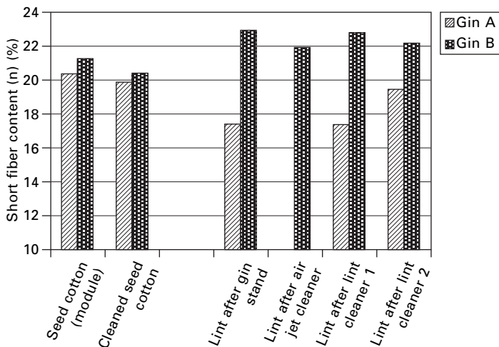
3.7 Short fiber content (n) of cotton processed in two different gins. Gin B, working with high productivity, produces a somewhat higher short fiber content than Gin A, operating with a lower productivity.
