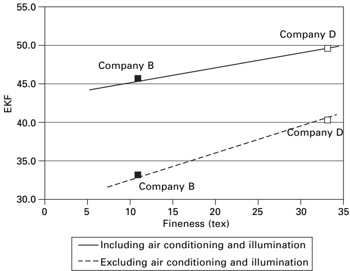
4.75 EKFs calculated with and without air conditioning and illumination.
