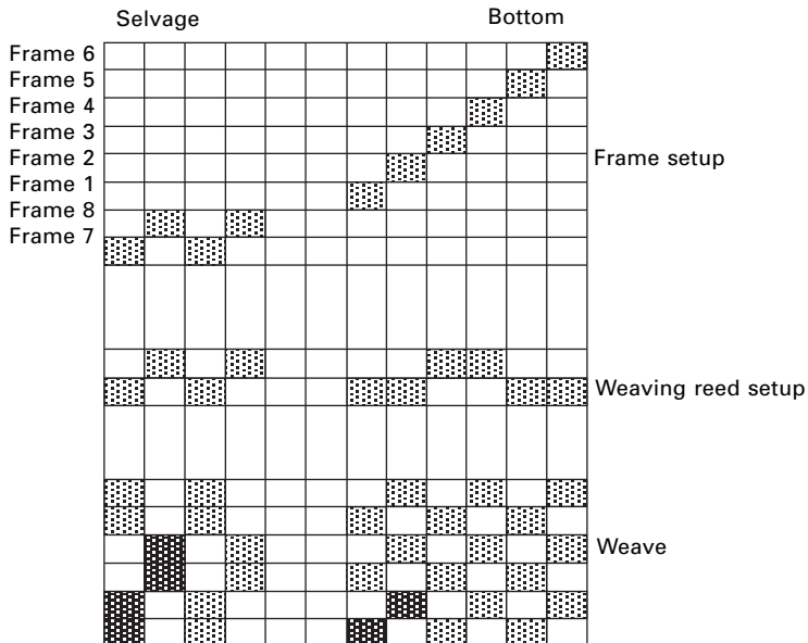
2.50 Example of machinery setup of a canvas fabric on a weaving machine.
