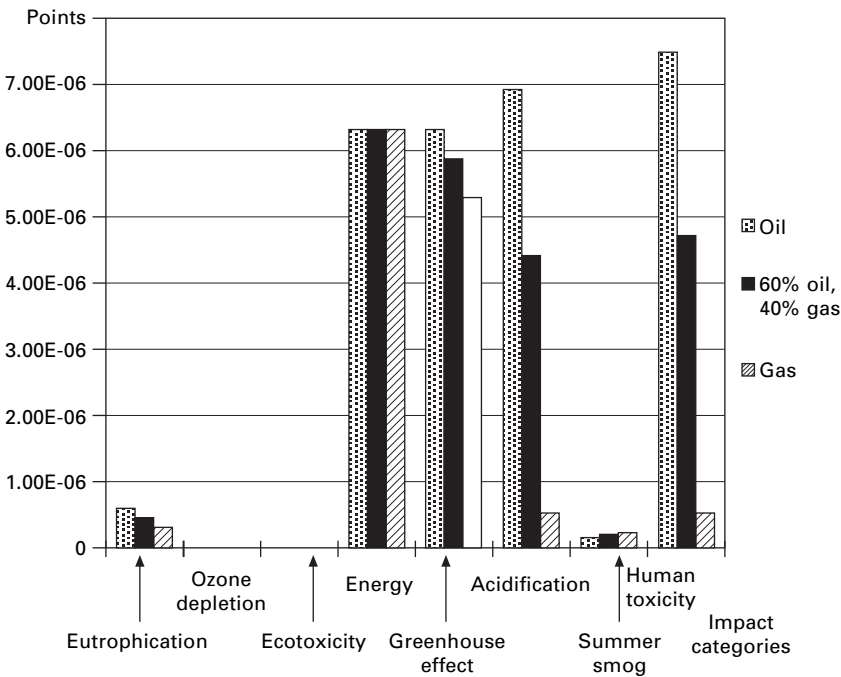
4.41 Scenarios for different prime sources (energy) in finishing (case study D).
