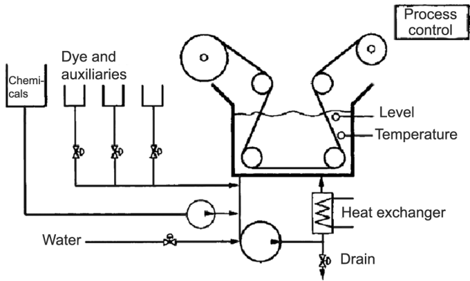
Schematic drawing of an automatic Jig
