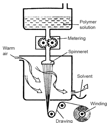
Dry spinning (schematic)
