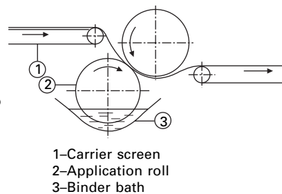
Applicator roll method
