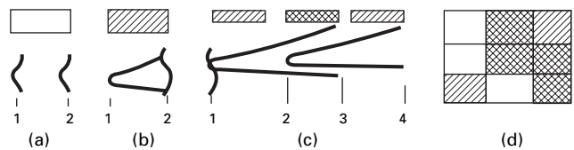
9.61 Deflection of guides (jacquard structure). (a) open structure, net opening is not covered by any underlap □ (b) semisolid structure, net opening is covered by two underlaps ▨ ; (c) solid structure, net opening is covered by four underlaps ▩ and (d) open, semisolid and solid structure.
