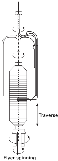
8.15 Two-for-one twisting (source: Grosberg and Ilye 1 ).
