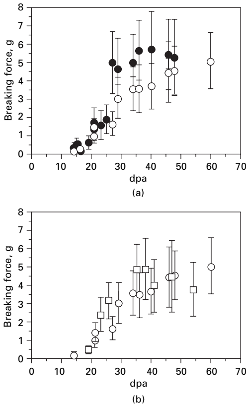
1.9 Single fiber breaking forces of developing G. hirsutum (SJ-2) cotton: (a) ● hydrated, ○ dried; (b) ○ random first-boll position from 6 plants, □ first-boll position from single plant.
