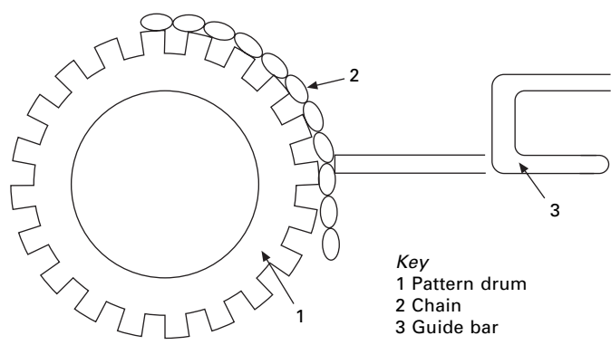
9.52 Pattern mechanism.
