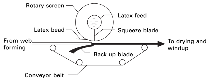
Latex printing process
