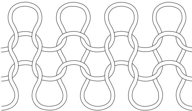
9.11 Rib fabric 1 × 1.
