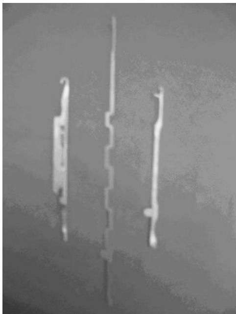
9.30 Latch needle.
