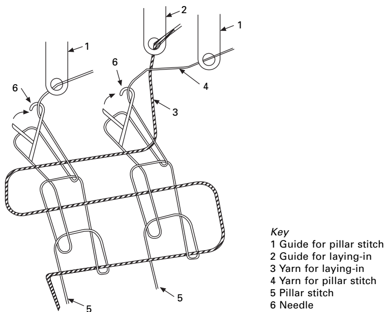
9.59 Laying-in movement.
