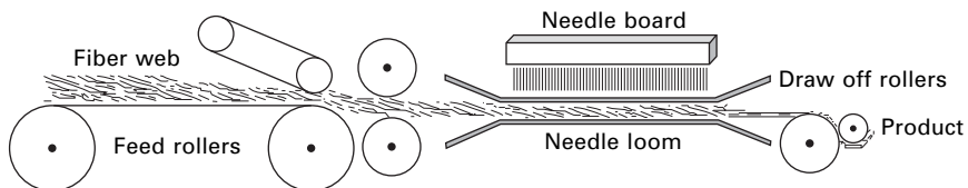
16.4 Schematic of the needle punching process (from ref. 4, with permission from INDIA).
