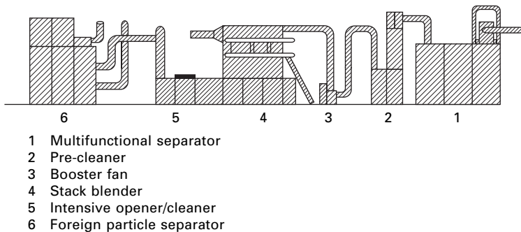
7.6 Sequence of machines comprising Stage 2.
