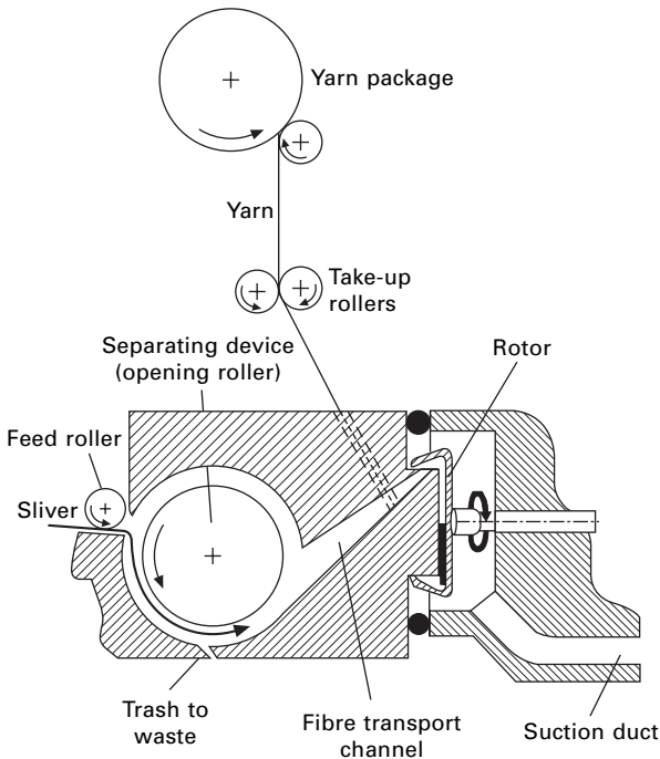
8.10 Open-end rotor spinning (source: Kwasniak and Peterson, J. Text. Inst. 88, (1/3), 174.
