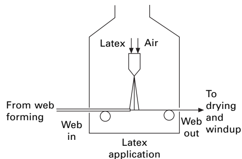
Schematic of spray bonding process
