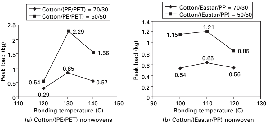
16.10 Effect of bonding temperature on (MD) strength of cotton-based nonwovens.
