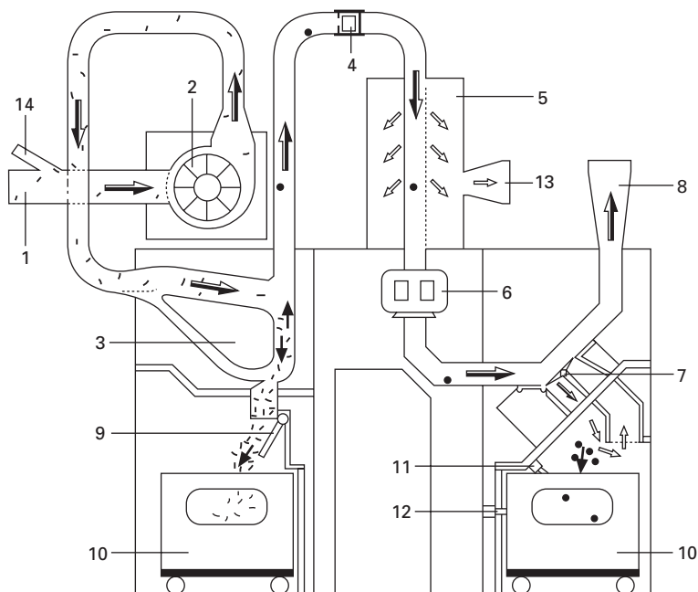
7.5 Multifunction Separator.
