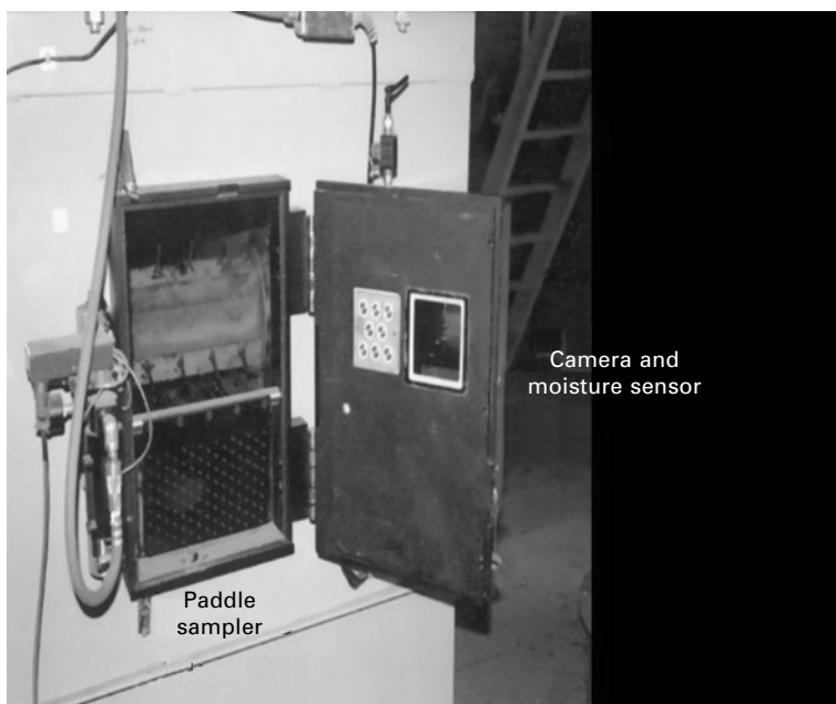
6.13 Typical sensing station used in the IntelliGin.
