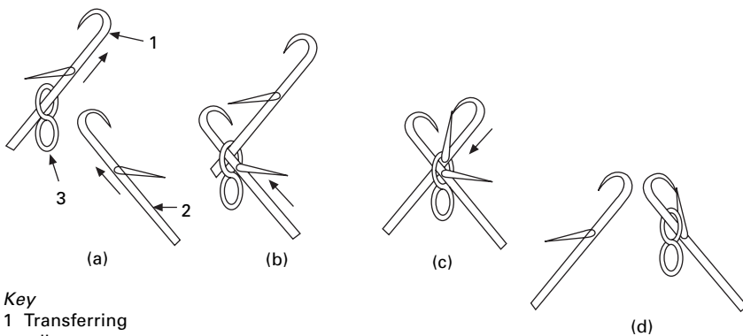
9.42 Transferred loop (a) beginning of transfer process, (b) receiving needle inserted into loop, (c) transferring needle begins decent and (d) transfer process completed.
