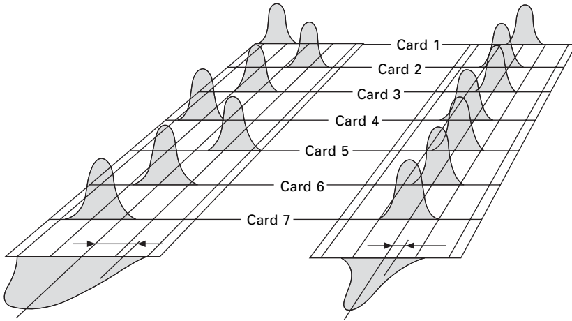
7.20 Count variations within and between cards.
