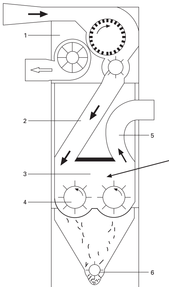
7.7 Opener/pre-cleaner.
