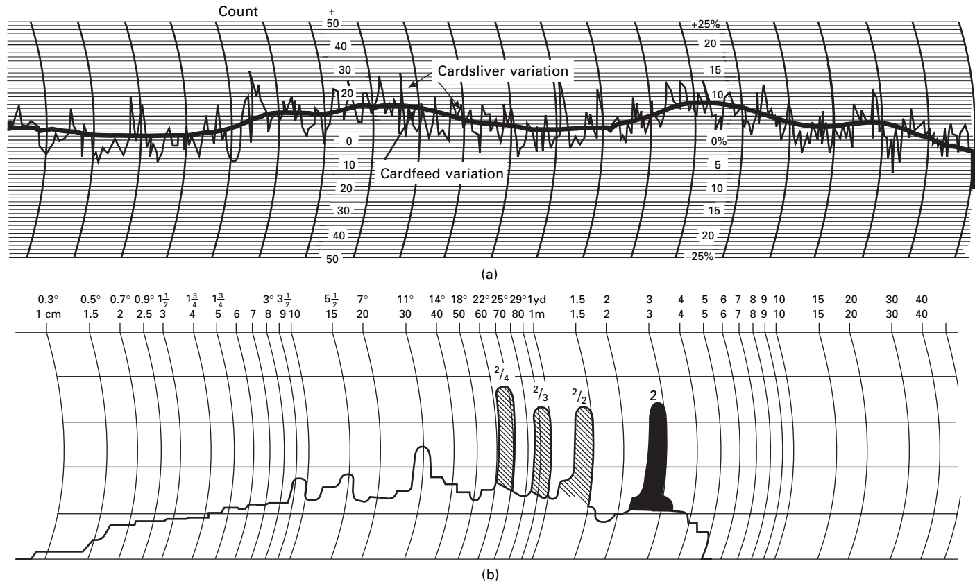
7.18 Irregularity trace and spectrograph of card sliver.
