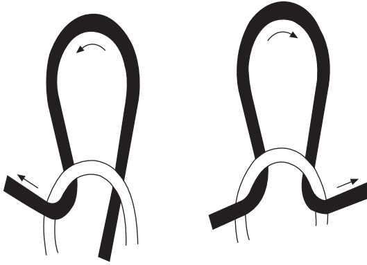
9.20 Open lap.
