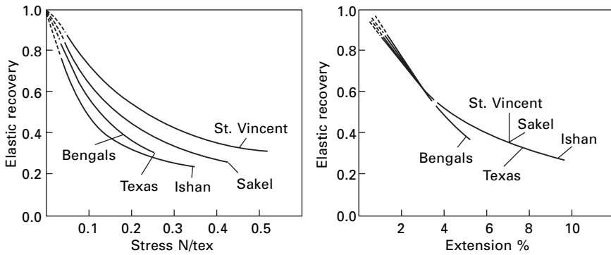
2.10 Elastic recovery of cottons plotted against stress and strain. From Meredith (1945b).
