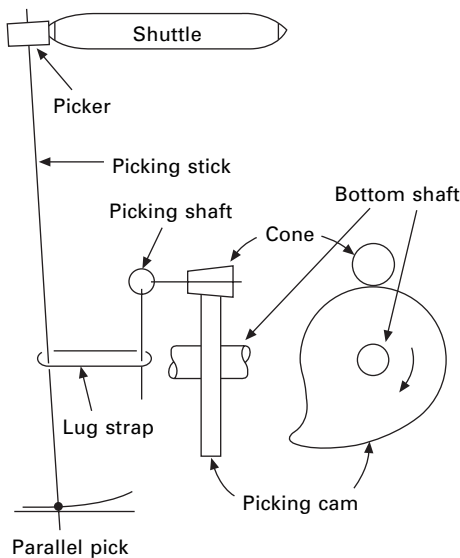
10.10 Cone-underpick.
