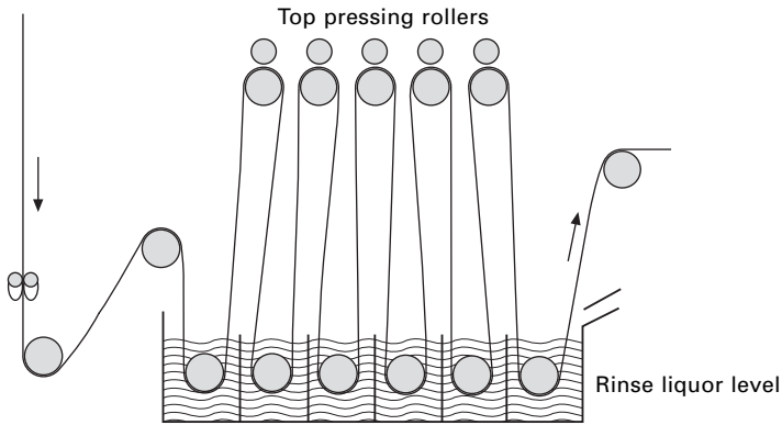
11.17 Wash-box.
