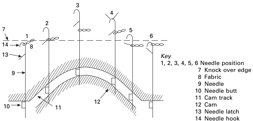
9.24 The needle position in cam track.
